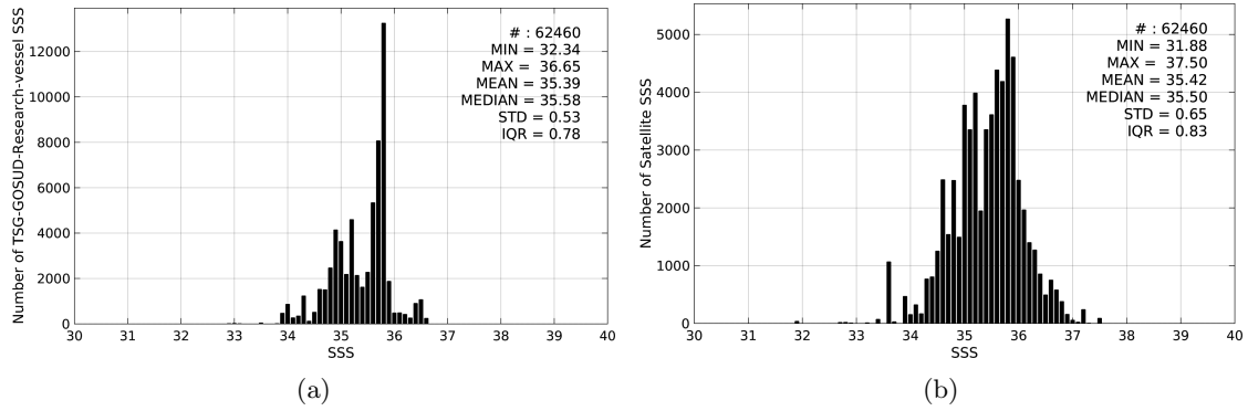
Figure 2: Histograms of SSS from TSG-GOSUD-Research-vessel (a) and SMOS-L3-CATDS-CECOS-IFREMER-V2-1DAY-0.5deg (b) considering all match-up pairs per bins of 0.1 over the South Pacific Ocean Pi-MEP region and for the full satellite product period.
