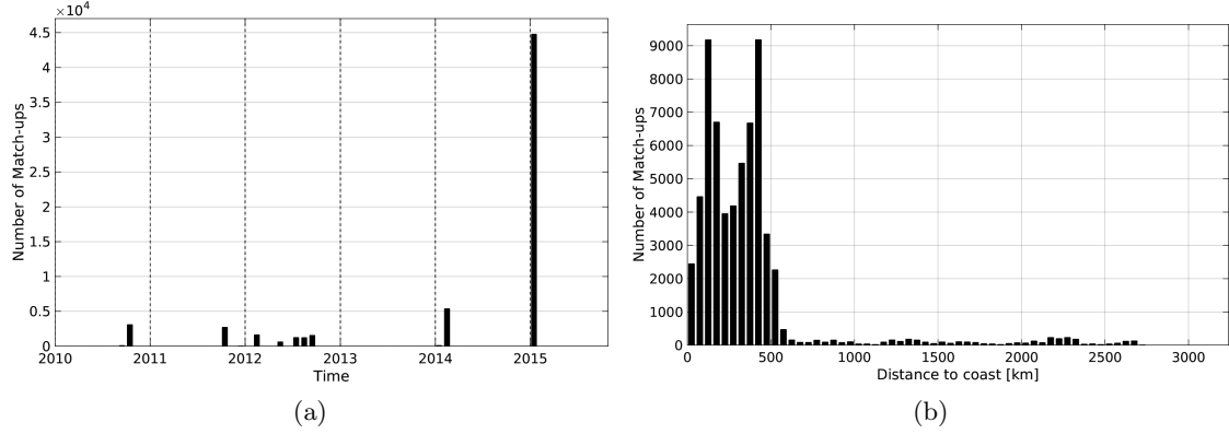
Figure 1: Number of match-ups between TSG-GOSUD-Research-vessel and SMOS-L3-CATDS-CECOS-IFREMER-V2-1DAY-0.5deg SSS as a function of time (a) and as function of the distance to coast (b) over the South Pacific Ocean Pi-MEP region and for the full satellite product period.
