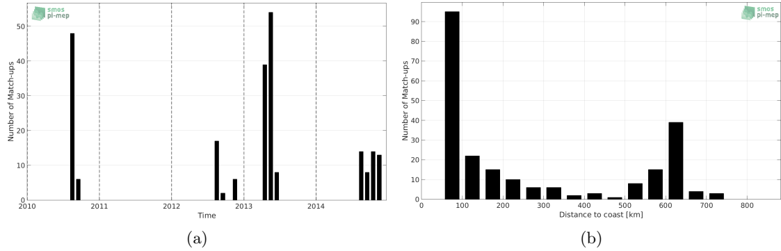
Figure 1: Number of match-ups between Sea mammals and SMOS-L3-CATDS-CECOS-IFREMER-V2-1DAY-0.5DEG SSS as a function of time (a) and as function of the distance to coast (b) over the South Pacific Ocean Pi-MEP region and for the full satellite product period.
