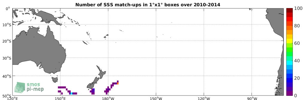
Figure 4: Number of SSS match-ups between Sea mammals SSS and the SMOS-L3-CATDS-CECOS-IFREMER-V2-1DAY-0.5DEG SSS product for the South Pacific Ocean Pi-MEP region over 1^{\circ} \times 1^{\circ} boxes and for the full satellite product period.
