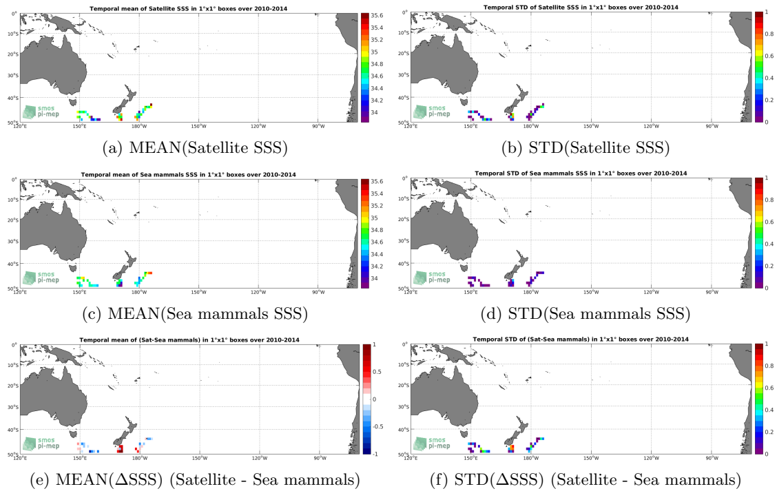
Figure 6: Temporal mean (left) and STD (right) of SSS from SMOS-L3-CATDS-CECOS-IFREMER-V2-1DAY-0.5DEG (top), Sea mammals (middle), and of \Delta SSS (Satellite - Sea mammals). Only match-up pairs are used to generate these maps.
