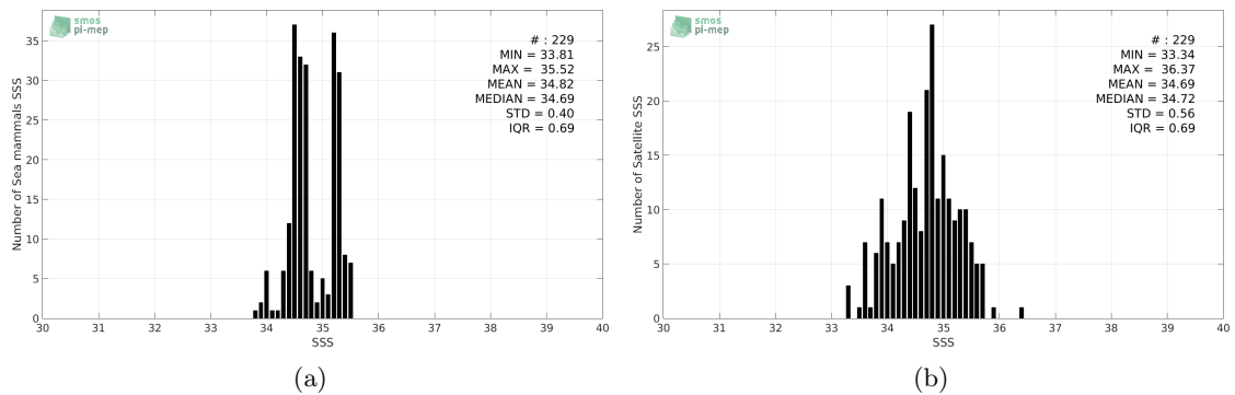
Figure 2: Histograms of SSS from Sea mammals (a) and SMOS-L3-CATDS-CECOS-IFREMER-V2-1DAY-0.5DEG (b) considering all match-up pairs per bins of 0.1 over the South Pacific Ocean Pi-MEP region and for the full satellite product period.
