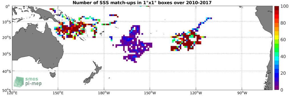
Figure 3: Number of SSS match-ups between Surface drifters SSS and the SMOS SSS L3 v2 - Daily - 0.5 Deg (CATDS-CECOS-IFREMER) SSS product for the South Pacific Ocean Pi-MEP region over 1^\circ \times 1^\circ boxes and for the full satellite product period.
