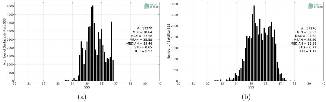
Figure 2: Histograms of SSS from Surface drifters (a) and SMOS SSS L3 v2 - Daily - 0.5 Deg (CATDS-CECOS-IFREMER) (b) considering all match-up pairs per bins of 0.1 over the South Pacific Ocean Pi-MEP region and for the full satellite product period.
