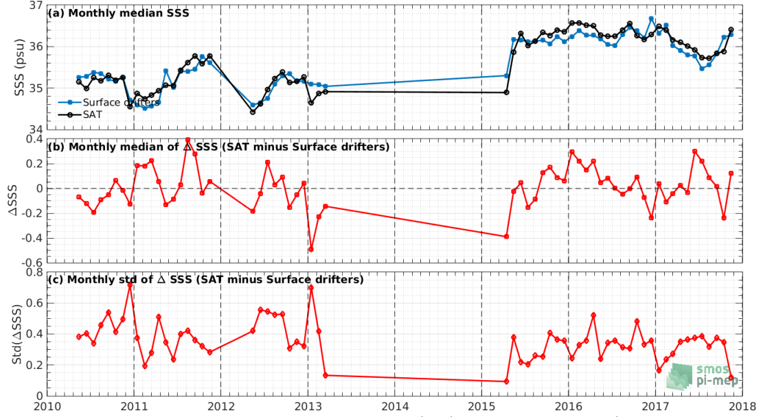
Figure 6: Time series of the monthly median SSS (top), median of \Delta\text{SSS} (Satellite - Surface drifters) and Std of \Delta\text{SSS} (Satellite - Surface drifters) over the South Pacific Ocean Pi-MEP region considering all match-ups collected by the Pi-MEP.
