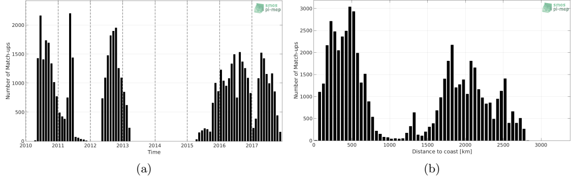
Figure 1: Number of match-ups between Surface drifters and SMOS SSS L3 v2 - Daily - 0.5 Deg (CATDS-CECOS-IFREMER) SSS as a function of time (a) and as function of the distance to coast (b) over the South Pacific Ocean Pi-MEP region and for the full satellite product period.
