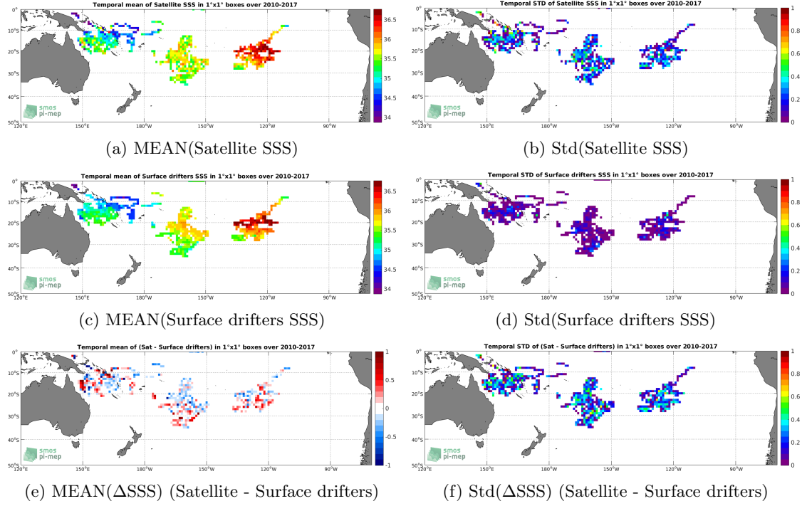
Figure 5: Temporal mean (left) and Std (right) of SSS from SMOS SSS L3 v2 - Daily - 0.5 Deg (CATDS-CECOS-IFREMER) (top), Surface drifters (middle), and of \Delta SSS (Satellite - Surface drifters). Only match-up pairs are used to generate these maps.
