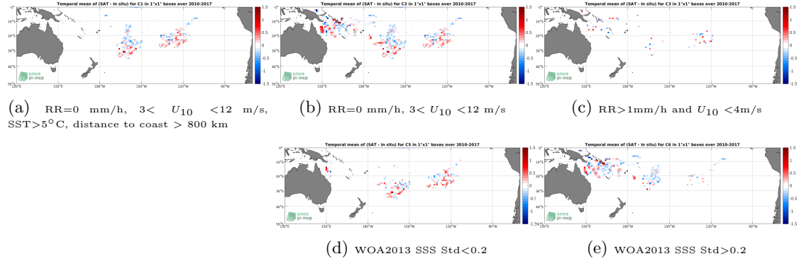
Figure 11: Temporal mean gridded over spatial boxes of size 1^{\circ}\times 1^{\circ} of \Delta\text{SSS} (SMOS SSS L3 v2 - Daily - 0.5 Deg (CATDS-CECOS-IFREMER) - Surface drifters) for 5 different subdatasets corresponding to: \text{RR}=0 mm/h, 3 < U_{10} < 12 m/s, SST > 5^{\circ}\text{C} , distance to coast > 800 km (a), \text{RR}=0 mm/h, 3 < U_{10} < 12 m/s (b), \text{RR} > 1\text{mm/h} and U_{10} < 4\text{m/s} (c), WOA2013 SSS Std < 0.2 (d), WOA2013 SSS Std > 0.2 (e).
