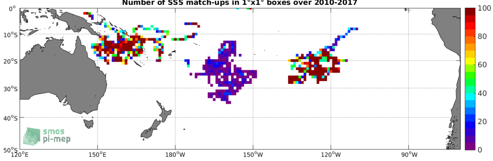
Figure 3: Number of SSS match-ups between Surface drifters SSS and the SMOS SSS L3 v2 - Daily - 0.5 Deg (CATDS-CECOS-IFREMER) SSS product for the South Pacific Ocean Pi-MEP region over 1°x1° boxes and for the full satellite product period.
