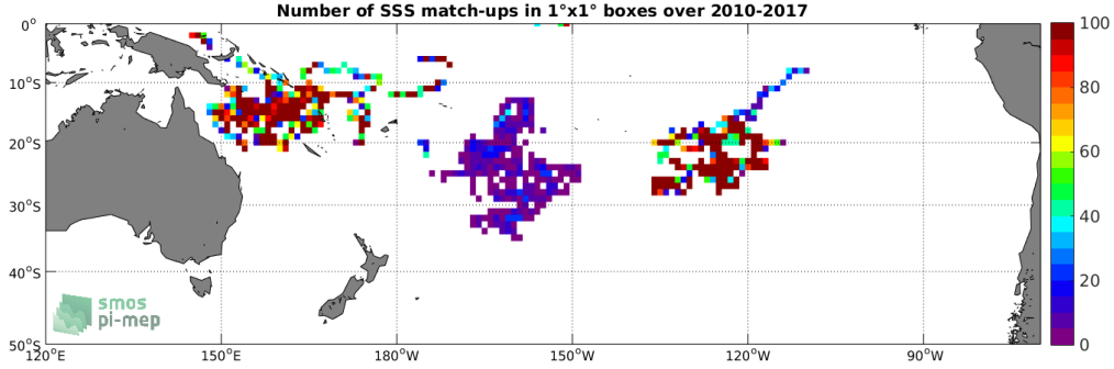
Figure 3: Number of SSS match-ups between Surface drifters SSS and the SMOS L3 v2 - Daily - 0.5 Deg (CATDS-CECOS-IFREMER) SSS product for the South Pacific Ocean Pi-MEP region over 1°x1° boxes and for the full satellite product period.
