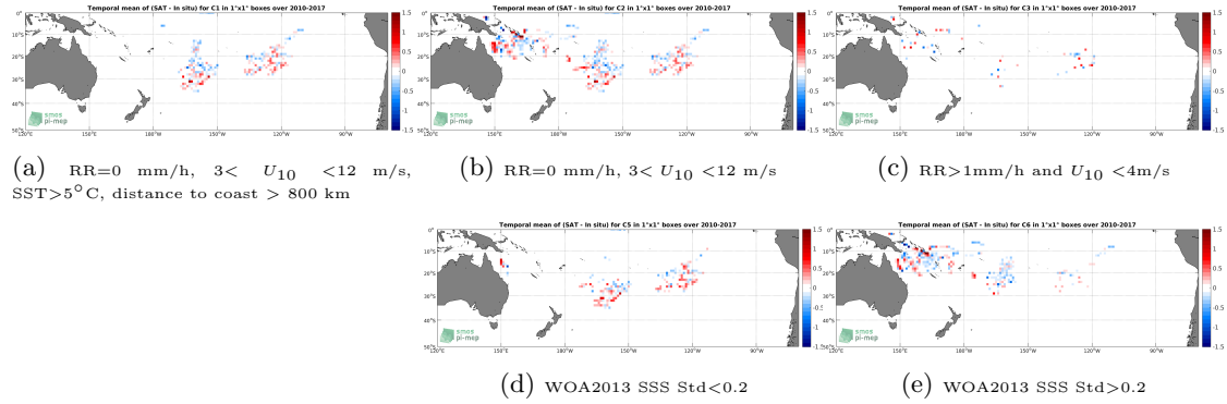
Figure 11: Temporal mean gridded over spatial boxes of size 1^{\circ}\times 1^{\circ} of \Delta\text{SSS} (SMOS L3 v2 - Daily - 0.5 Deg (CATDS-CECOS-IFREMER) - Surface drifters) for 5 different subdatasets corresponding to: \text{RR}=0 mm/h, 3 < U_{10} < 12 m/s, SST > 5^{\circ}\text{C} , distance to coast > 800 km (a), \text{RR}=0 mm/h, 3 < U_{10} < 12 m/s (b), \text{RR} > 1 mm/h and U_{10} < 4 m/s (c), WOA2013 SSS Std < 0.2 (d), WOA2013 SSS Std > 0.2 (e).
