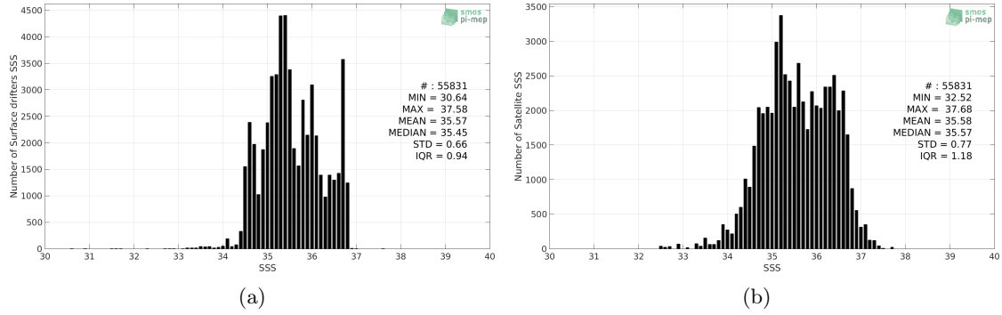
Figure 2: Histograms of SSS from Surface drifters (a) and SMOS L3 v2 - Daily - 0.5 Deg (CATDS-CECOS-IFREMER) (b) considering all match-up pairs per bins of 0.1 over the South Pacific Ocean Pi-MEP region and for the full satellite product period.
