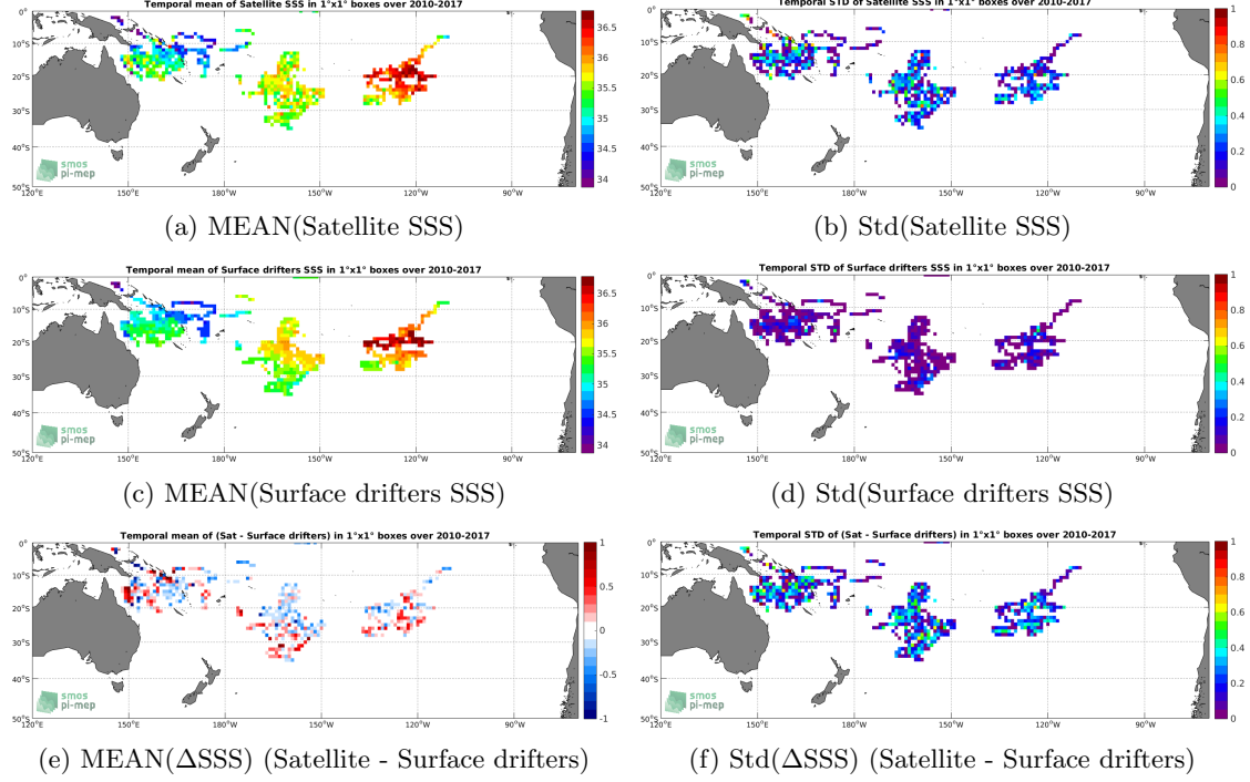
Figure 5: Temporal mean (left) and Std (right) of SSS from SMOS L3 v2 - Daily - 0.5 Deg (CATDS-CECOS-IFREMER) (top), Surface drifters (middle), and of \Delta SSS (Satellite - Surface drifters). Only match-up pairs are used to generate these maps.
