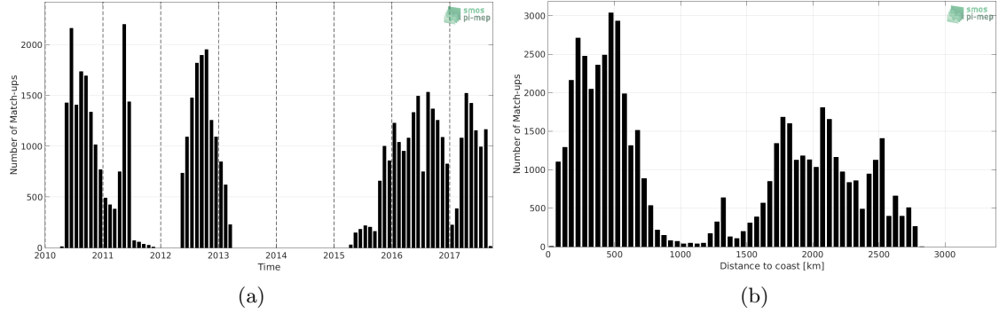
Figure 1: Number of match-ups between Surface drifters and SMOS L3 v2 - Daily - 0.5 Deg (CATDS-CECOS-IFREMER) SSS as a function of time (a) and as function of the distance to coast (b) over the South Pacific Ocean Pi-MEP region and for the full satellite product period.
