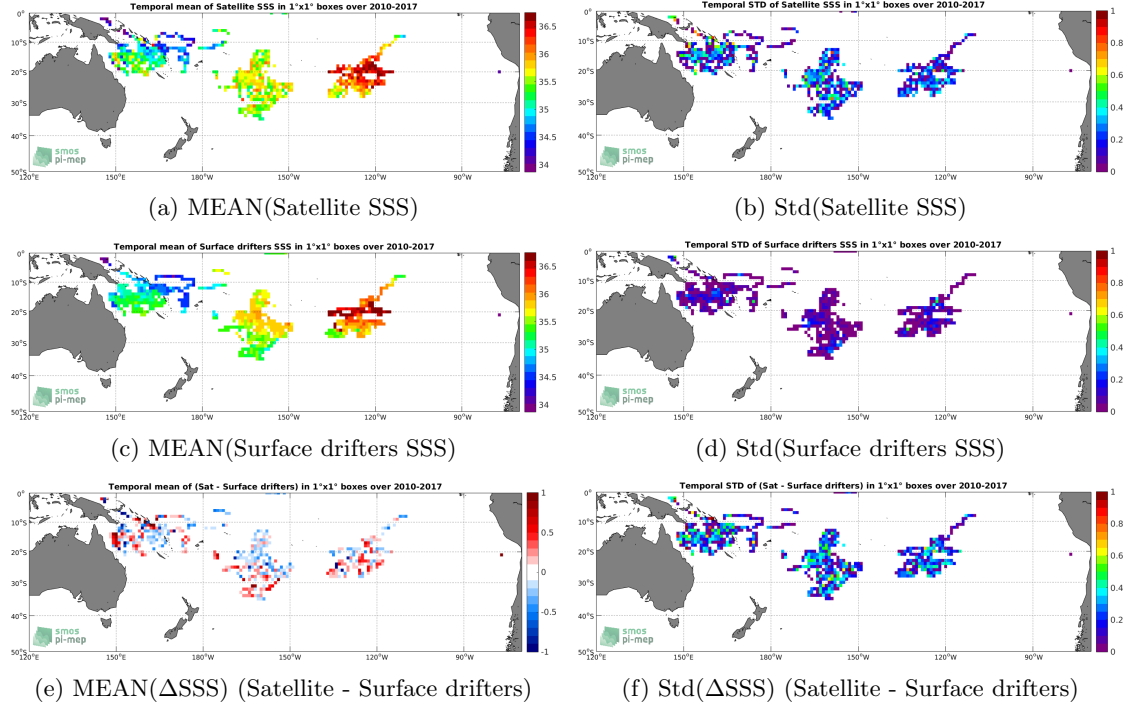
Figure 5: Temporal mean (left) and Std (right) of SSS from SMOS-L3-CATDS-CECOS-IFREMER-V2-1DAY-0.5DEG (top), Surface drifters (middle), and of \Delta SSS (Satellite - Surface drifters). Only match-up pairs are used to generate these maps.
