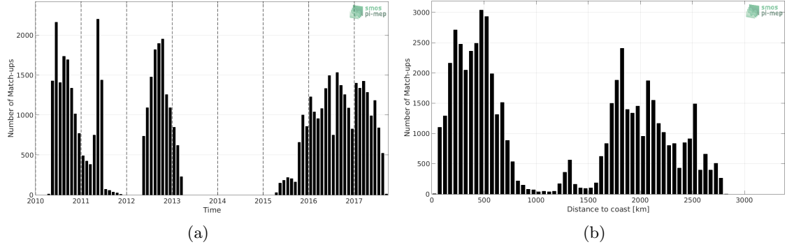
Figure 1: Number of match-ups between Surface drifters and SMOS-L3-CATDS-CECOS-IFREMER-V2-1DAY-0.5DEG SSS as a function of time (a) and as function of the distance to coast (b) over the South Pacific Ocean Pi-MEP region and for the full satellite product period.
