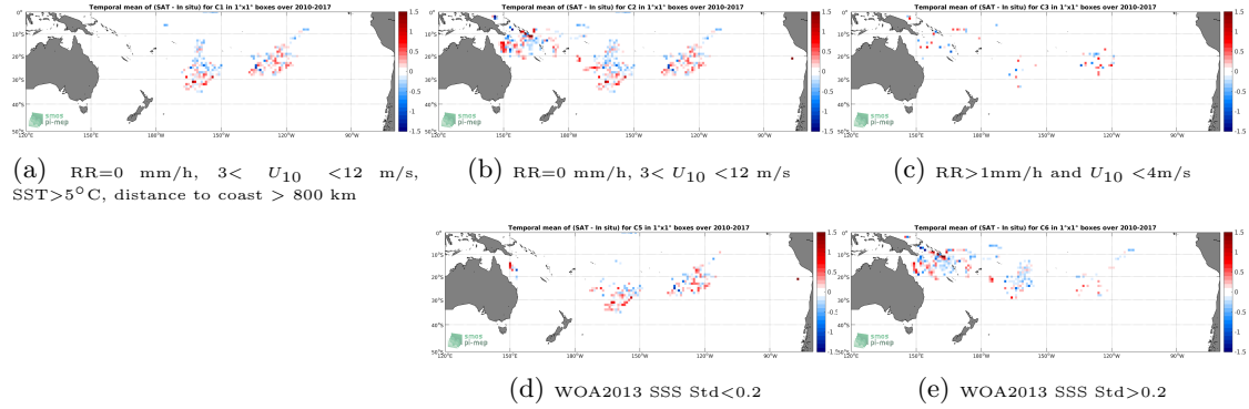
Figure 11: Temporal mean gridded over spatial boxes of size 1^\circ \times 1^\circ of \Delta SSS (SMOS-L3-CATDS-CECOS-IFREMER-V2-1DAY-0.5DEG - Surface drifters) for 5 different subdatasets corresponding to: RR=0 mm/h, 3 < U_{10} < 12 m/s, SST > 5^\circ\text{C} , distance to coast > 800 km (a), RR=0 mm/h, 3 < U_{10} < 12 m/s (b), RR > 1 mm/h and U_{10} < 4 m/s (c), WOA2013 SSS Std < 0.2 (d), WOA2013 SSS Std > 0.2 (e).
