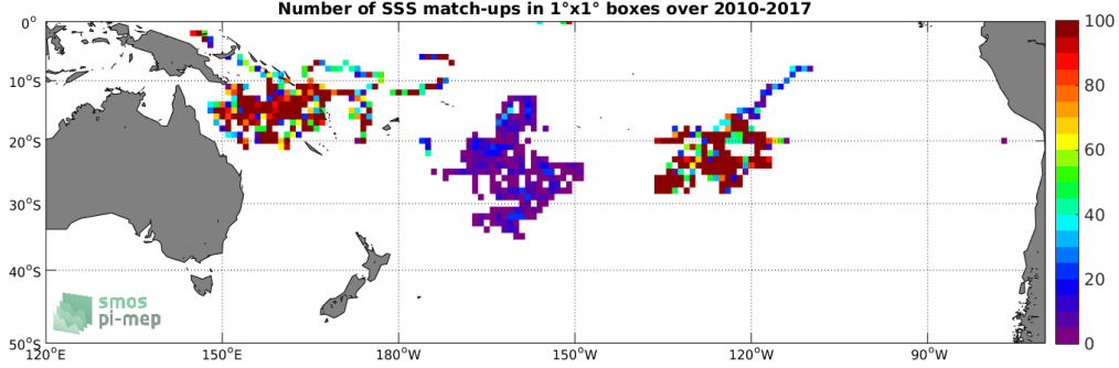
Figure 3: Number of SSS match-ups between Surface drifters SSS and the SMOS-L3-CATDS-CECOS-IFREMER-V2-1DAY-0.5DEG SSS product for the South Pacific Ocean Pi-MEP region over 1°x1° boxes and for the full satellite product period.
