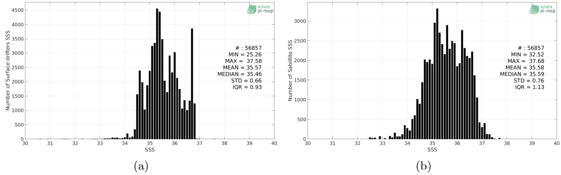
Figure 2: Histograms of SSS from Surface drifters (a) and SMOS-L3-CATDS-CECOS-IFREMER-V2-1DAY-0.5DEG (b) considering all match-up pairs per bins of 0.1 over the South Pacific Ocean Pi-MEP region and for the full satellite product period.
