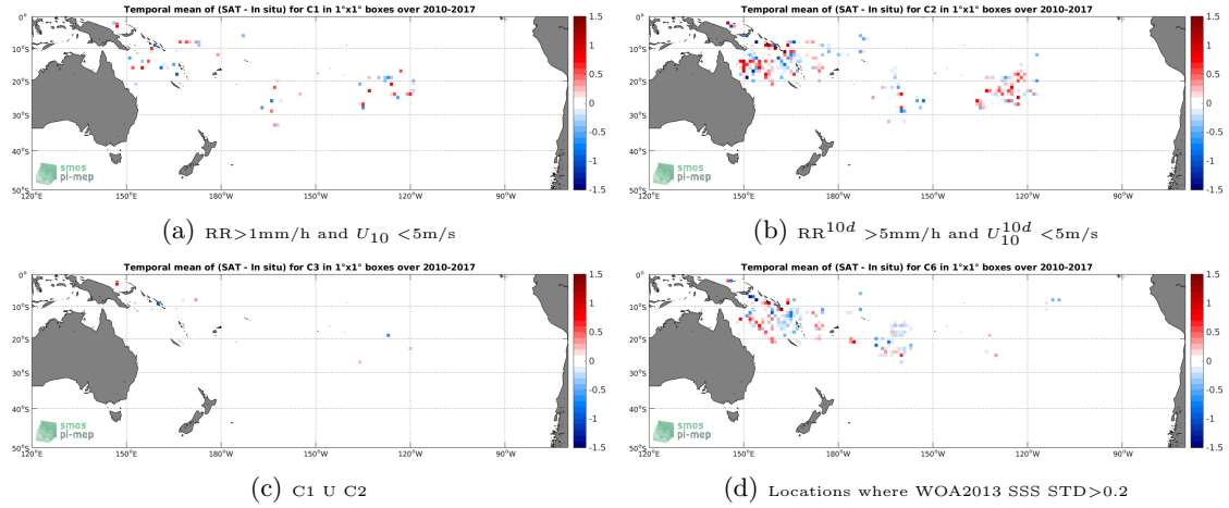
Figure 11: Temporal mean gridded over spatial boxes of size 1^\circ \times 1^\circ of \Delta SSS (SMOS-L3-CATDS-CECOS-IFREMER-V2-1DAY-0.5DEG - Surface drifters) for 4 different subdatasets corresponding to: RR > 1\text{mm/h} and U_{10} < 5\text{m/s} (a), RR^{10d} > 5\text{mm/h} and U_{10}^{10d} < 5\text{m/s} (b), C1 U C2 (c), Locations where WOA2013 SSS STD > 0.2 (d).
