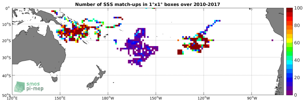
Figure 3: Number of SSS match-ups between Surface drifters SSS and the SMOS-L3-CATDS-CECOS-IFREMER-V2-1DAY-0.5DEG SSS product for the South Pacific Ocean Pi-MEP region over 1^\circ \times 1^\circ boxes and for the full satellite product period.
