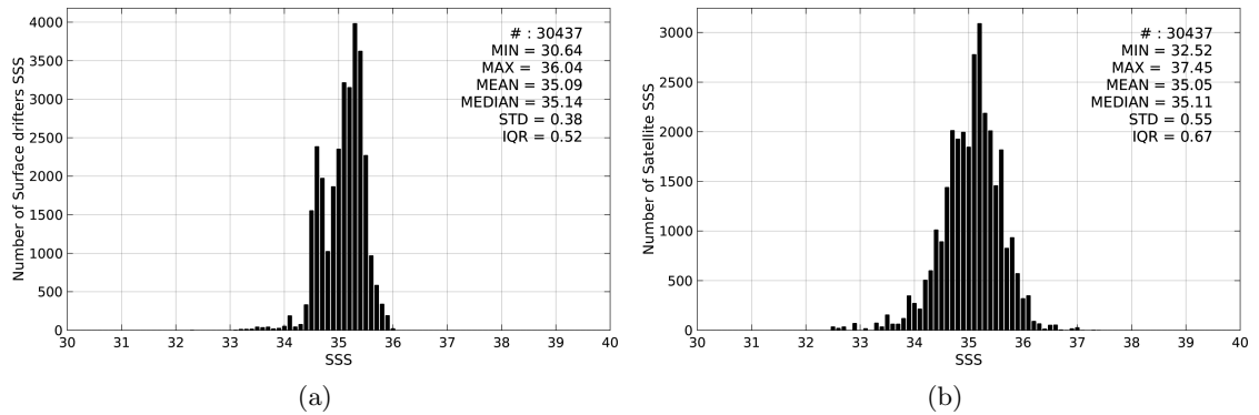
Figure 2: Histograms of SSS from Surface drifters (a) and SMOS-L3-CATDS-CECOS-IFREMER-V2-1DAY-0.5DEG (b) considering all match-up pairs per bins of 0.1 over the South Pacific Ocean Pi-MEP region and for the full satellite product period.
