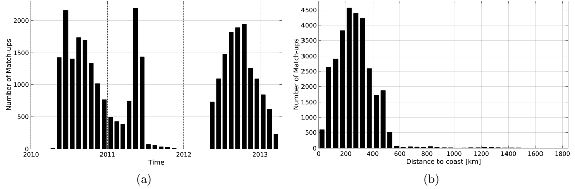
Figure 1: Number of match-ups between Surface drifters and SMOS-L3-CATDS-CECOS-IFREMER-V2-1DAY-0.5DEG SSS as a function of time (a) and as function of the distance to coast (b) over the South Pacific Ocean Pi-MEP region and for the full satellite product period.
