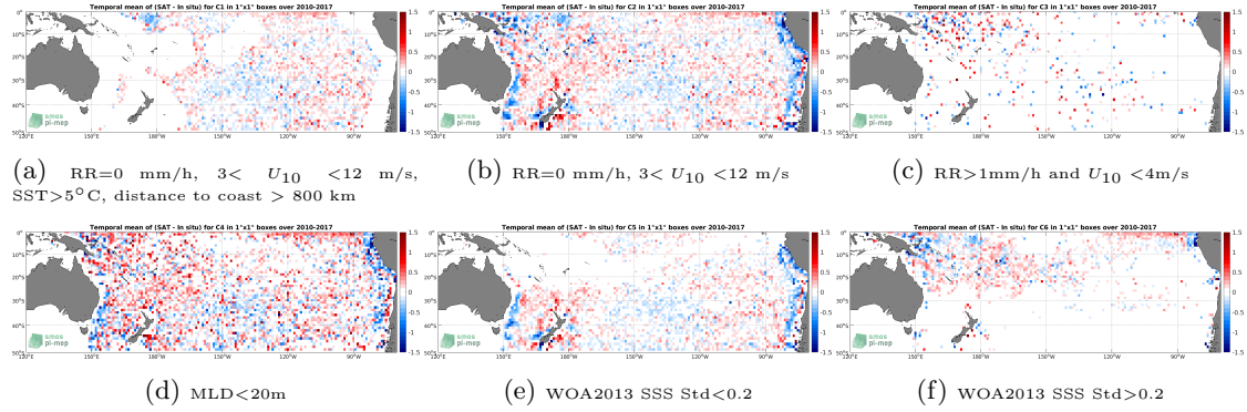
Figure 12: Temporal mean gridded over spatial boxes of size 1^\circ \times 1^\circ of \Delta SSS (SMOS SSS L3 v2 - Daily - 0.5 Deg (CATDS-CECOS-IFREMER) - Argo) for 6 different subdatasets corresponding to:RR=0 mm/h, 3 < U_{10} < 12 m/s, SST >5^\circ\text{C} , distance to coast > 800 km (a), RR=0 mm/h, 3 < U_{10} < 12 m/s (b), RR >1 mm/h and U_{10} < 4 m/s (c),MLD <20 m (d),WOA2013 SSS Std <0.2 (e),WOA2013 SSS Std >0.2 (f).
