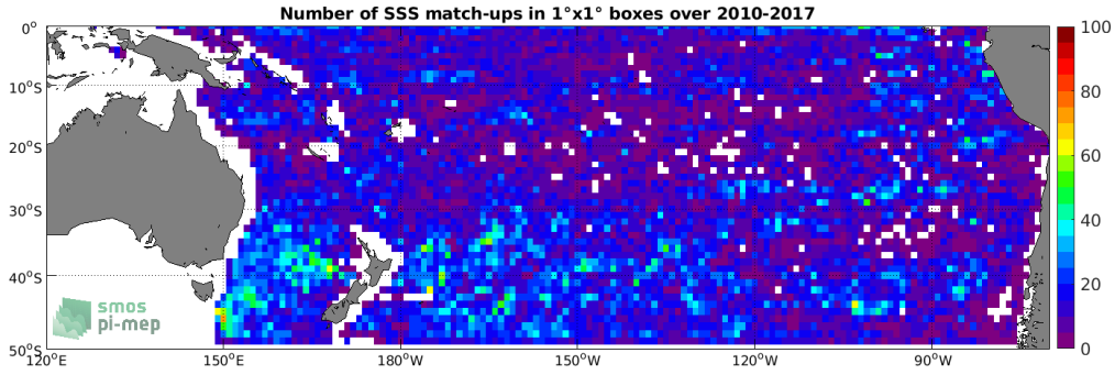
Figure 4: Number of SSS match-ups between Argo SSS and the SMOS SSS L3 v2 - Daily - 0.5 Deg (CATDS-CECOS-IFREMER) SSS product for the South Pacific Ocean Pi-MEP region over 1^\circ \times 1^\circ boxes and for the full satellite product period.
