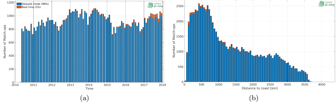
Figure 1: Number of match-ups between Argo and SMOS SSS L3 v2 - Daily - 0.5 Deg (CATDS-CECOS-IFREMER) SSS as a function of time (a) and as function of the distance to coast (b) over the South Pacific Ocean Pi-MEP region and for the full satellite product period.
