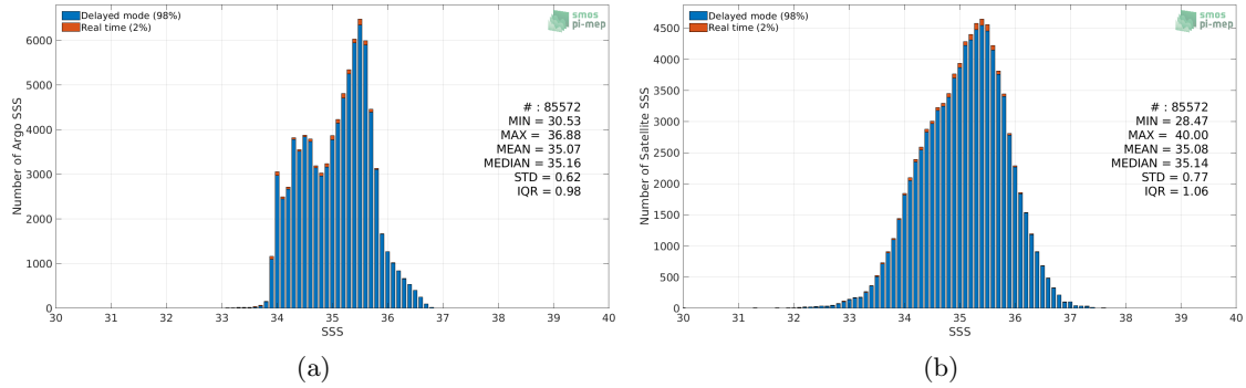
Figure 2: Histograms of SSS from Argo (a) and SMOS SSS L3 v2 - Daily - 0.5 Deg (CATDS-CECOS-IFREMER) (b) considering all match-up pairs per bins of 0.1 over the South Pacific Ocean Pi-MEP region and for the full satellite product period.
