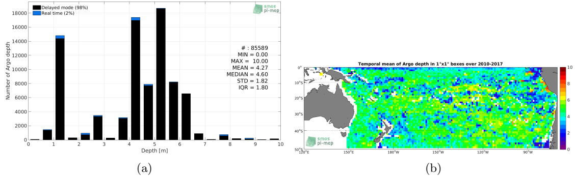
Figure 3: Histograms of the depth of the upper level SSS measurements from Argo in the Match-up DataBase for the South Pacific Ocean Pi-MEP region (a) and temporal mean spatial distribution of pressure of the in situ SSS data over 1^\circ \times 1^\circ boxes and for the full satellite product period (b).
