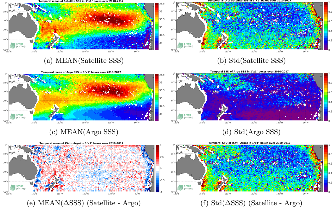
Figure 6: Temporal mean (left) and Std (right) of SSS from SMOS-L3-CATDS-CECOS-IFREMER-V2-1DAY-0.5DEG (top), Argo (middle), and of \Delta SSS (Satellite - Argo). Only match-up pairs are used to generate these maps.
