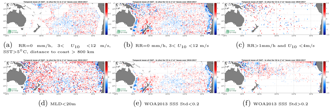
Figure 12: Temporal mean gridded over spatial boxes of size 1^\circ \times 1^\circ of \Delta SSS (SMOS-L3-CATDS-CECOS-IFREMER-V2-1DAY-0.5DEG - Argo) for 6 different subdatasets corresponding to: RR=0 mm/h, 3 < U_{10} < 12 m/s, SST > 5^\circ C , distance to coast > 800 km (a), RR=0 mm/h, 3 < U_{10} < 12 m/s (b), RR > 1 mm/h and U_{10} < 4 m/s (c), MLD < 20 m (d), WOA2013 SSS Std < 0.2 (e), WOA2013 SSS Std > 0.2 (f).
