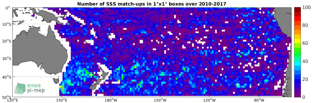
Figure 4: Number of SSS match-ups between Argo SSS and the SMOS-L3-CATDS-CECOS-IFREMER-V2-1DAY-0.5DEG SSS product for the South Pacific Ocean Pi-MEP region over 1^\circ \times 1^\circ boxes and for the full satellite product period.
