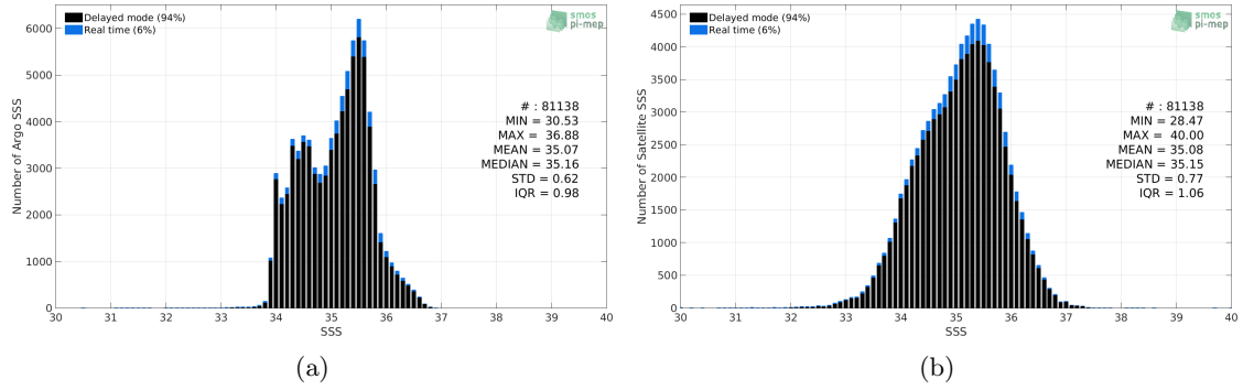
Figure 2: Histograms of SSS from Argo (a) and SMOS-L3-CATDS-CECOS-IFREMER-V2-1DAY-0.5DEG (b) considering all match-up pairs per bins of 0.1 over the South Pacific Ocean Pi-MEP region and for the full satellite product period.
