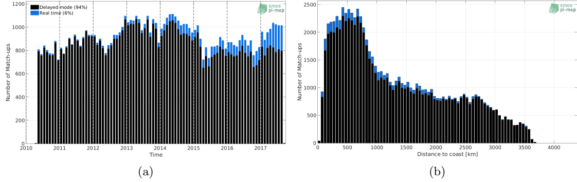
Figure 1: Number of match-ups between Argo and SMOS-L3-CATDS-CECOS-IFREMER-V2-1DAY-0.5DEG SSS as a function of time (a) and as function of the distance to coast (b) over the South Pacific Ocean Pi-MEP region and for the full satellite product period.
