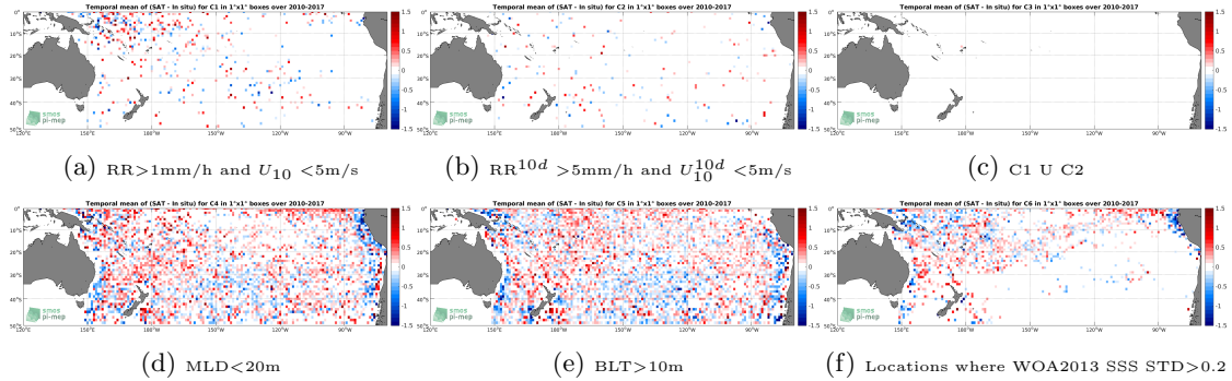
Figure 12: Temporal mean gridded over spatial boxes of size 1°x1° of \Delta SSS (SMOS-L3-CATDS-CECOS-IFREMER-V2-1DAY-0.5DEG - Argo) for 6 different subdatasets corresponding to:RR>1mm/h and U_{10} < 5m/s (a), RR^{10d} > 5mm/h and U_{10}^{10d} < 5m/s (b), C1 U C2 (c),MLD<20m (d),BLT>10m (e),Locations where WOA2013 SSS STD>0.2 (f).
