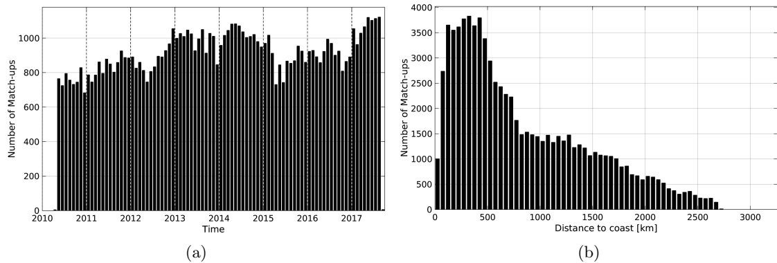
Figure 1: Number of match-ups between Argo and SMOS-L3-CATDS-CECOS-IFREMER-V2-1DAY-0.5DEG SSS as a function of time (a) and as function of the distance to coast (b) over the South Pacific Ocean Pi-MEP region and for the full satellite product period.
