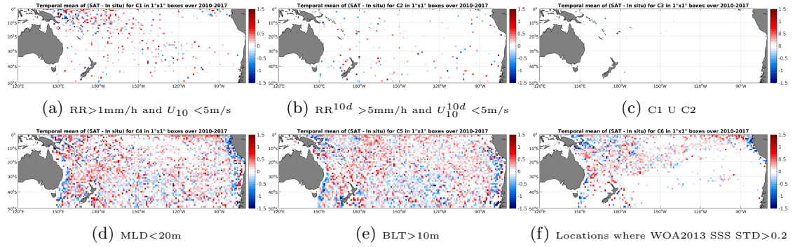
Figure 12: Temporal mean gridded over spatial boxes of size 1^\circ \times 1^\circ of \Delta SSS (SMOS-L3-CATDS-CECOS-IFREMER-V2-1DAY-0.5DEG - Argo) for 6 different subdatasets corresponding to: RR > 1mm/h and U_{10} < 5 m/s (a), RR^{10d} > 5 mm/h and U_{10}^{10d} < 5 m/s (b), C1 U C2 (c), MLD < 20m (d), BLT > 10m (e), Locations where WOA2013 SSS STD > 0.2 (f).
