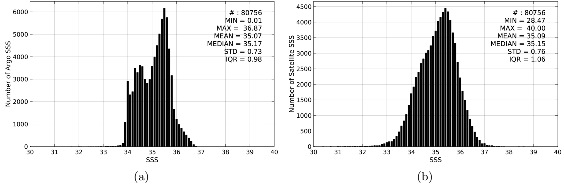
Figure 2: Histograms of SSS from Argo (a) and SMOS-L3-CATDS-CECOS-IFREMER-V2-1DAY-0.5DEG (b) considering all match-up pairs per bins of 0.1 over the South Pacific Ocean Pi-MEP region and for the full satellite product period.
