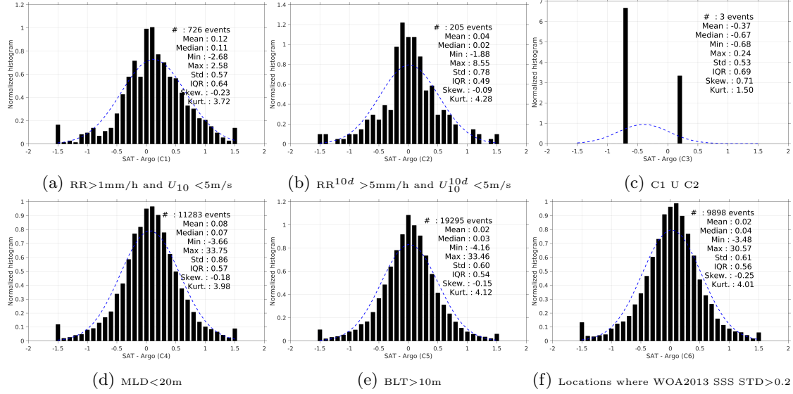
Figure 13: Normalized histogram of \Delta\text{SSS} (SMOS-L3-CATDS-CECOS-IFREMER-V2-1DAY-0.5deg - Argo) for 6 different subdatasets corresponding to: \text{RR} > 1\text{mm/h} and U_{10} < 5\text{m/s} (a), \text{RR}^{10d} > 5\text{mm/h} and U_{10}^{10d} < 5\text{m/s} (b), C1 U C2 (c), \text{MLD} < 20\text{m} (d), \text{BLT} > 10\text{m} (e), Locations where WOA2013 SSS STD > 0.2 (f).
