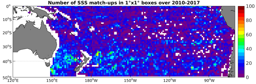
Figure 4: Number of SSS match-ups between Argo SSS and the SMOS-L3-CATDS-CECOS-IFREMER-V2-1DAY-0.5deg SSS product for the South Pacific Ocean Pi-MEP region over 1°x1° boxes and for the full satellite product period.
