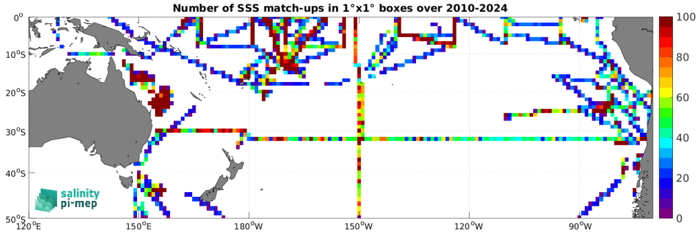
Figure 5: Number of SSS match-ups between TSG (SAMOS) SSS and the SMOS SSS L3 v335 - Monthly - 25 km (CATDS-CPDC) SSS product for the South Pacific Ocean Pi-MEP region over 1^\circ \times 1^\circ boxes and for the full satellite product period.
