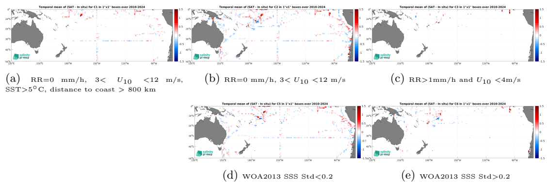
Figure 14: Temporal mean gridded over spatial boxes of size 1^\circ \times 1^\circ of \Delta\text{SSS} (SMOS SSS L3 v335 - Monthly - 25 km (CATDS-CPDC) - TSG (SAMOS)) for 5 different subdatasets corresponding to:RR=0 mm/h, 3 < U_{10} < 12 m/s, SST>5°C, distance to coast > 800 km (a), RR=0 mm/h, 3 < U_{10} < 12 m/s (b), RR>1mm/h and U_{10} < 4 m/s (c), WOA2013 SSS Std<0.2 (d), WOA2013 SSS Std>0.2 (e).
