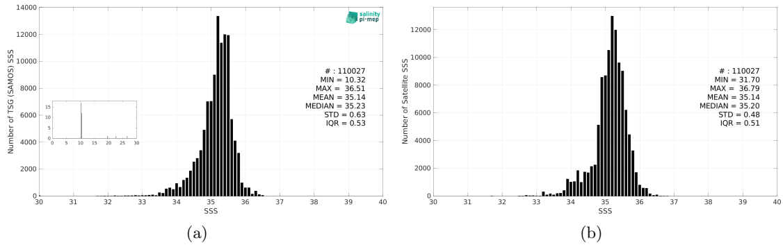
Figure 3: Histograms of SSS from TSG (SAMOS) (a) and SMOS SSS L3 v335 - Monthly - 25 km (CATDS-CPDC) (b) considering all match-up pairs per bins of 0.1 over the South Pacific Ocean Pi-MEP region and for the full satellite product period.
