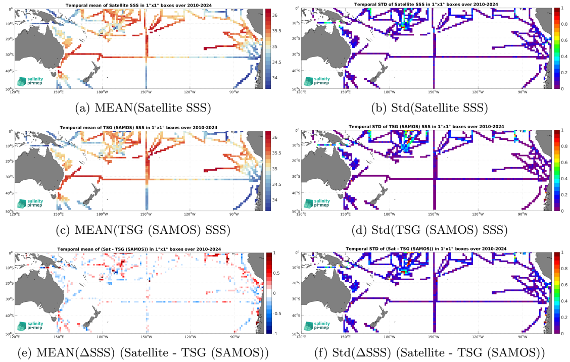
Figure 7: Temporal mean (left) and Std (right) of SSS from SMOS SSS L3 v335 - Monthly - 25 km (CATDS-CPDC) (top), TSG (SAMOS) (middle), and of \Delta SSS (Satellite - TSG (SAMOS)). Only match-up pairs are used to generate these maps.
