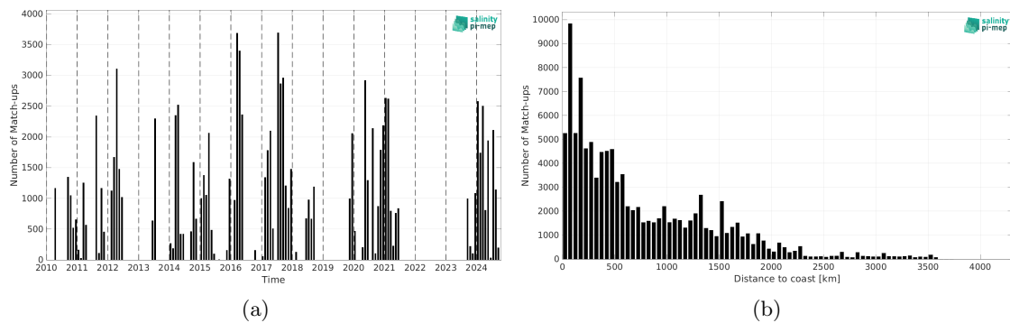
Figure 2: Number of match-ups between TSG (SAMOS) and SMOS SSS L3 v335 - Monthly - 25 km (CATDS-CPDC) SSS as a function of time (a) and as function of the distance to coast (b) over the South Pacific Ocean Pi-MEP region and for the full satellite product period.
