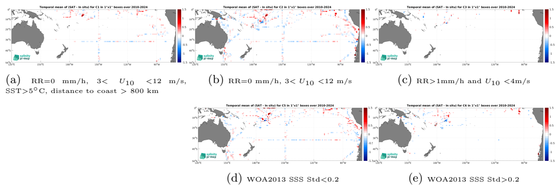
Figure 14: Temporal mean gridded over spatial boxes of size 1^\circ \times 1^\circ of \Delta SSS (SMOS SSS L3 v335 - Monthly - 25 km (CATDS-CPDC) - TSG (SAMOS)) for 5 different subdatasets corresponding to:RR=0 mm/h, 3 < U_{10} < 12 m/s, SST >5^\circ C, distance to coast > 800 km (a), RR=0 mm/h, 3 < U_{10} < 12 m/s (b), RR >1 mm/h and U_{10} < 4 m/s (c), WOA2013 SSS Std <0.2 (d), WOA2013 SSS Std >0.2 (e).
