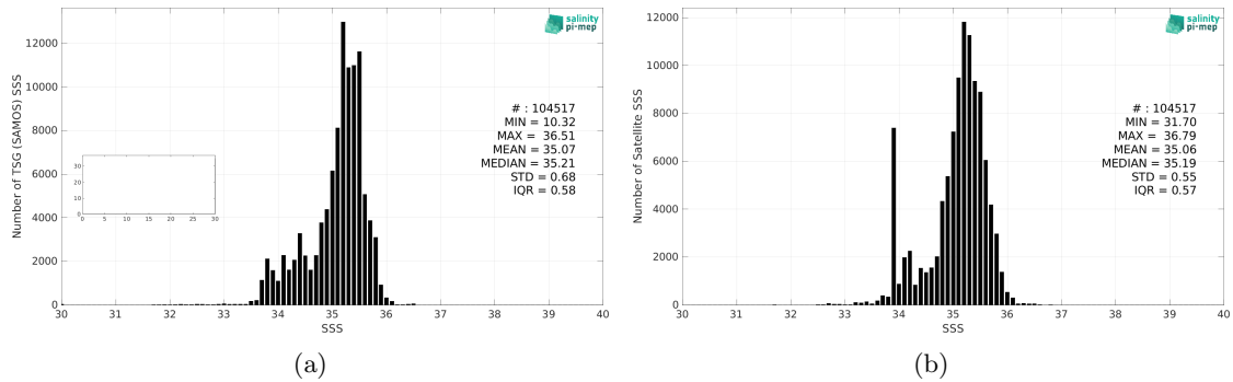
Figure 2: Histograms of SSS from TSG (SAMOS) (a) and SMOS SSS L3 v335 - Monthly - 25 km (CATDS-CPDC) (b) considering all match-up pairs per bins of 0.1 over the South Pacific Ocean Pi-MEP region and for the full satellite product period.
