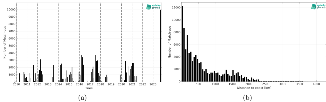
Figure 1: Number of match-ups between TSG (SAMOS) and SMOS SSS L3 v335 - Monthly - 25 km (CATDS-CPDC) SSS as a function of time (a) and as function of the distance to coast (b) over the South Pacific Ocean Pi-MEP region and for the full satellite product period.
