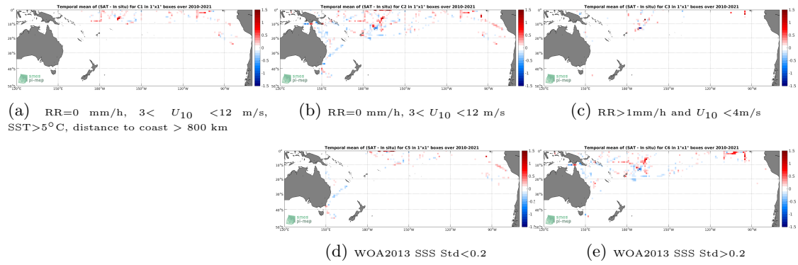
Figure 12: Temporal mean gridded over spatial boxes of size 1^\circ \times 1^\circ of \Delta SSS (SMOS SSS L3 v335 - Monthly - 25 km (CATDS-CPDC) - TSG (SAMOS)) for 5 different subdatasets corresponding to:RR=0 mm/h, 3 < U_{10} < 12 m/s, SST >5^\circ\text{C} , distance to coast > 800 km (a), RR=0 mm/h, 3 < U_{10} < 12 m/s (b), RR >1 mm/h and U_{10} < 4 m/s (c), WOA2013 SSS Std <0.2 (d), WOA2013 SSS Std >0.2 (e).
