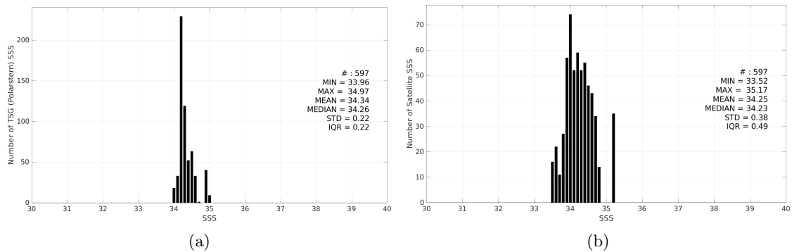
Figure 3: Histograms of SSS from TSG (Polarstern) (a) and SMOS SSS L3 v335 - Monthly - 25 km (CATDS-CPDC) (b) considering all match-up pairs per bins of 0.1 over the South Pacific Ocean Pi-MEP region and for the full satellite product period.
