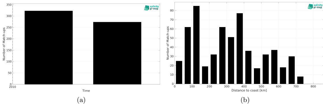
Figure 2: Number of match-ups between TSG (Polarstern) and SMOS SSS L3 v335 - Monthly - 25 km (CATDS-CPDC) SSS as a function of time (a) and as function of the distance to coast (b) over the South Pacific Ocean Pi-MEP region and for the full satellite product period.
