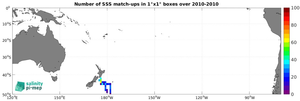
Figure 5: Number of SSS match-ups between TSG (Polarstern) SSS and the SMOS SSS L3 v335 - Monthly - 25 km (CATDS-CPDC) SSS product for the South Pacific Ocean Pi-MEP region over 1^\circ \times 1^\circ boxes and for the full satellite product period.
