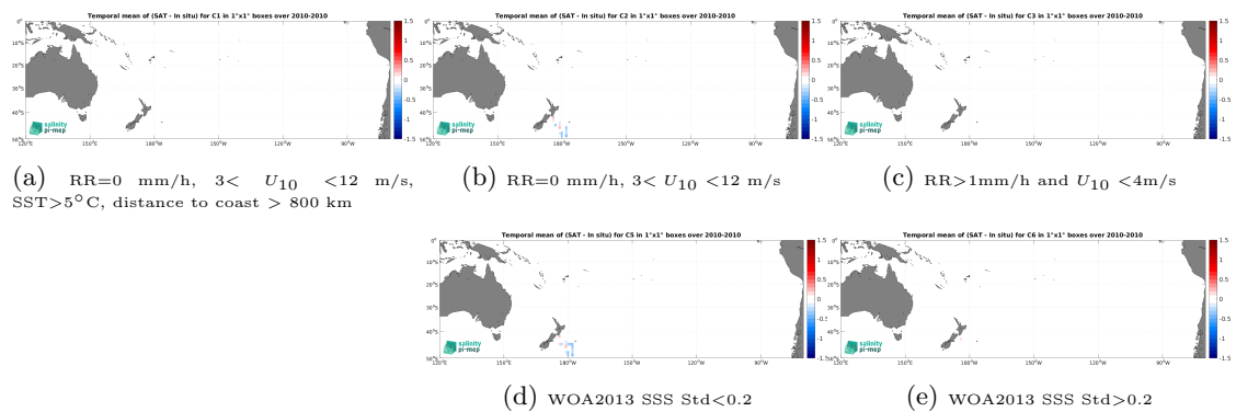
Figure 14: Temporal mean gridded over spatial boxes of size 1^\circ \times 1^\circ of \Delta SSS (SMOS SSS L3 v335 - Monthly - 25 km (CATDS-CPDC) - TSG (Polarstern)) for 5 different subdatasets corresponding to:RR=0 mm/h, 3 < U_{10} < 12 m/s, SST>5°C, distance to coast > 800 km (a), RR=0 mm/h, 3 < U_{10} < 12 m/s (b), RR>1mm/h and U_{10} < 4 m/s (c), WOA2013 SSS Std<0.2 (d), WOA2013 SSS Std>0.2 (e).
