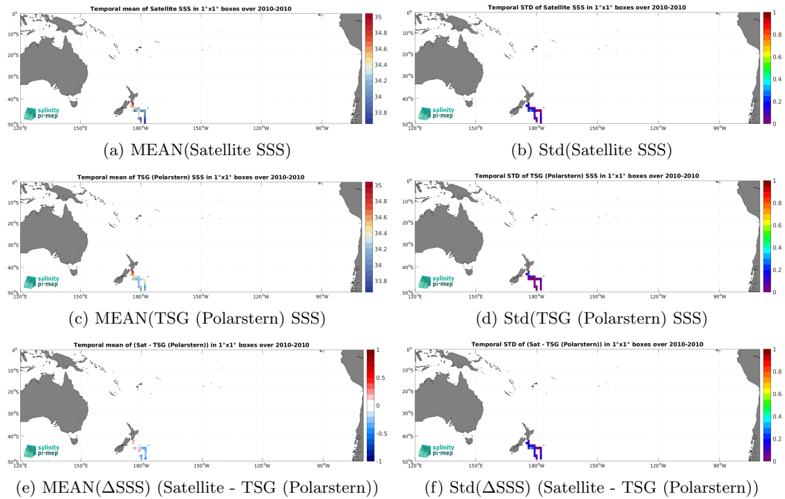
Figure 7: Temporal mean (left) and Std (right) of SSS from SMOS SSS L3 v335 - Monthly - 25 km (CATDS-CPDC) (top), TSG (Polarstern) (middle), and of \Delta SSS (Satellite - TSG (Polarstern)). Only match-up pairs are used to generate these maps.
