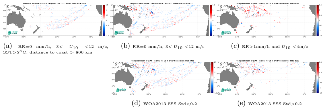
Figure 14: Temporal mean gridded over spatial boxes of size 1^\circ \times 1^\circ of \Delta SSS (SMOS SSS L3 v335 - Monthly - 25 km (CATDS-CPDC) - TSG (LEGOS-DM)) for 5 different subdatasets corresponding to:RR=0 mm/h, 3 < U_{10} < 12 m/s, SST >5^\circ\text{C} , distance to coast > 800 km (a), RR=0 mm/h, 3 < U_{10} < 12 m/s (b), RR >1 mm/h and U_{10} < 4 m/s (c), WOA2013 SSS Std <0.2 (d), WOA2013 SSS Std >0.2 (e).
