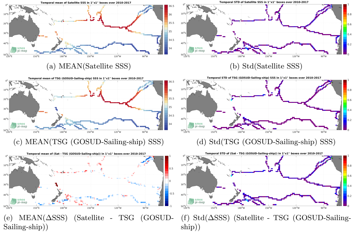
Figure 6: Temporal mean (left) and Std (right) of SSS from SMOS SSS L3 v335 - Monthly - 25 km (CATDS-CPDC) (top), TSG (GOSUD-Sailing-ship) (middle), and of \Delta SSS (Satellite - TSG (GOSUD-Sailing-ship)). Only match-up pairs are used to generate these maps.
