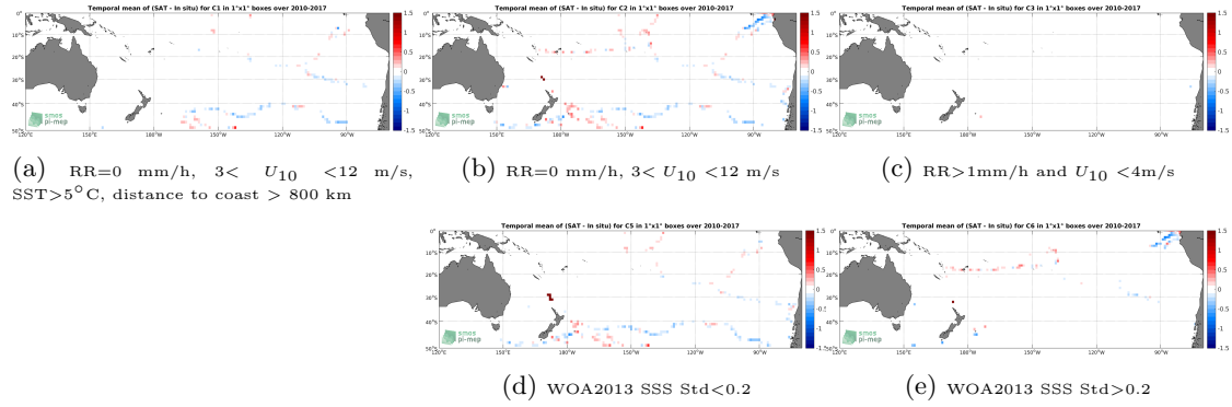
Figure 12: Temporal mean gridded over spatial boxes of size 1^\circ \times 1^\circ of \Delta SSS (SMOS SSS L3 v335 - Monthly - 25 km (CATDS-CPDC) - TSG (GOSUD-Sailing-ship)) for 5 different subdatasets corresponding to:RR=0 mm/h, 3 < U_{10} < 12 m/s, SST >5^\circ\text{C} , distance to coast > 800 km (a), RR=0 mm/h, 3 < U_{10} < 12 m/s (b), RR >1\text{mm/h} and U_{10} < 4\text{m/s} (c), WOA2013 SSS Std <0.2 (d), WOA2013 SSS Std >0.2 (e).
