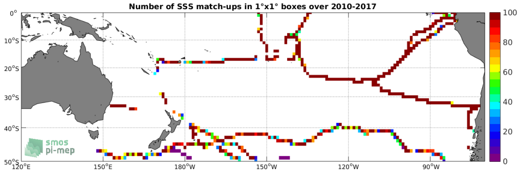
Figure 4: Number of SSS match-ups between TSG (GOSUD-Sailing-ship) SSS and the SMOS SSS L3 v335 - Monthly - 25 km (CATDS-CPDC) SSS product for the South Pacific Ocean Pi-MEP region over 1^\circ \times 1^\circ boxes and for the full satellite product period.
