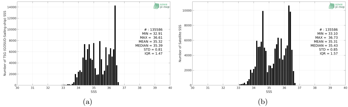
Figure 2: Histograms of SSS from TSG (GOSUD-Sailing-ship) (a) and SMOS SSS L3 v335 - Monthly - 25 km (CATDS-CPDC) (b) considering all match-up pairs per bins of 0.1 over the South Pacific Ocean Pi-MEP region and for the full satellite product period.
