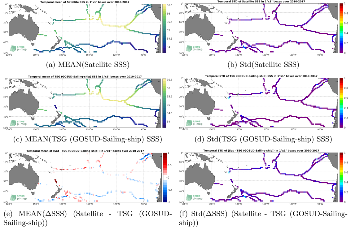
Figure 6: Temporal mean (left) and Std (right) of SSS from SMOS SSS L3 v335 - Monthly - 25 km (CATDS-CPDC) (top), TSG (GOSUD-Sailing-ship) (middle), and of \Delta SSS (Satellite - TSG (GOSUD-Sailing-ship)). Only match-up pairs are used to generate these maps.
