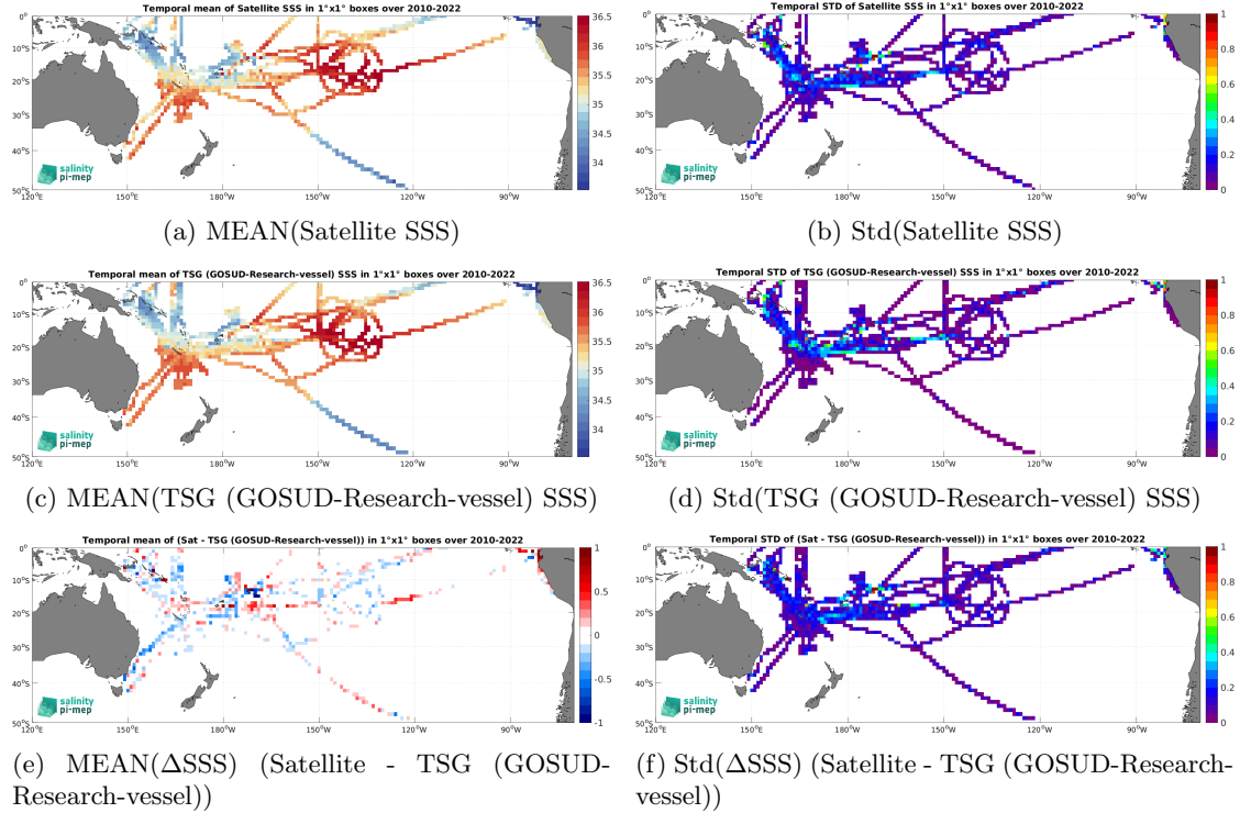
Figure 7: Temporal mean (left) and Std (right) of SSS from SMOS SSS L3 v335 - Monthly - 25 km (CATDS-CPDC) (top), TSG (GOSUD-Research-vessel) (middle), and of \Delta SSS (Satellite - TSG (GOSUD-Research-vessel)). Only match-up pairs are used to generate these maps.
