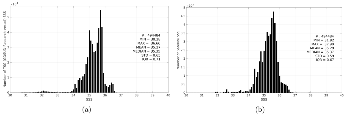
Figure 3: Histograms of SSS from TSG (GOSUD-Research-vessel) (a) and SMOS SSS L3 v335 - Monthly - 25 km (CATDS-CPDC) (b) considering all match-up pairs per bins of 0.1 over the South Pacific Ocean Pi-MEP region and for the full satellite product period.
