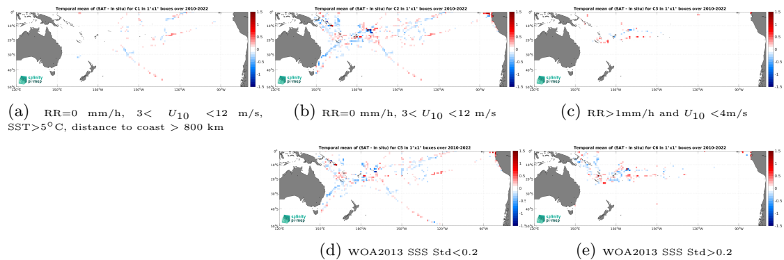
Figure 14: Temporal mean gridded over spatial boxes of size 1^\circ \times 1^\circ of \Delta SSS (SMOS SSS L3 v335 - Monthly - 25 km (CATDS-CPDC) - TSG (GOSUD-Research-vessel)) for 5 different subdatasets corresponding to:RR=0 mm/h, 3 < U_{10} < 12 m/s, SST >5^\circ C, distance to coast > 800 km (a), RR=0 mm/h, 3 < U_{10} < 12 m/s (b), RR >1 mm/h and U_{10} < 4 m/s (c), WOA2013 SSS Std <0.2 (d), WOA2013 SSS Std >0.2 (e).
