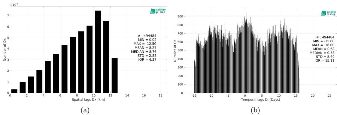
Figure 6: Histograms of the spatial (a) and temporal (b) lags between the location/time of the TSG (GOSUD-Research-vessel) measurement and the date of the corresponding SMOS SSS L3 v335 - Monthly - 25 km (CATDS-CPDC) SSS pixel.
