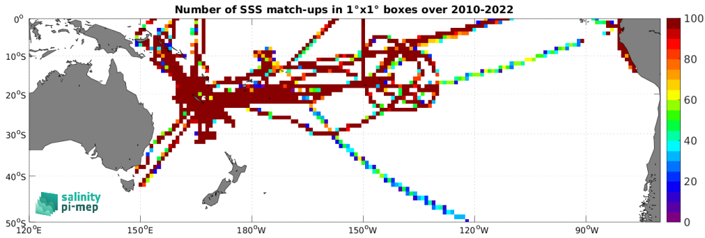
Figure 5: Number of SSS match-ups between TSG (GOSUD-Research-vessel) SSS and the SMOS SSS L3 v335 - Monthly - 25 km (CATDS-CPDC) SSS product for the South Pacific Ocean Pi-MEP region over 1^\circ \times 1^\circ boxes and for the full satellite product period.
