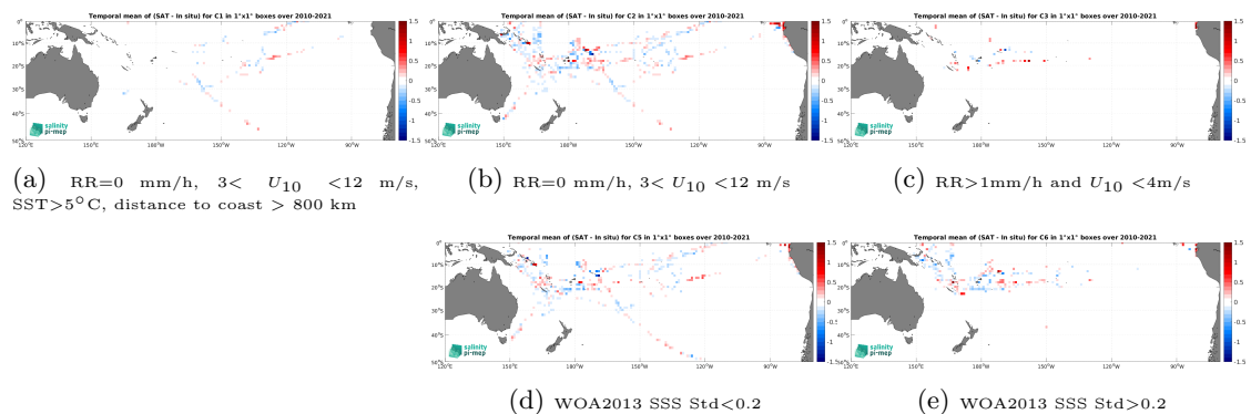
Figure 14: Temporal mean gridded over spatial boxes of size 1^\circ \times 1^\circ of \Delta\text{SSS} (SMOS SSS L3 v335 - Monthly - 25 km (CATDS-CPDC) - TSG (GOSUD-Research-vessel)) for 5 different subdatasets corresponding to:RR=0 mm/h, 3 < U_{10} < 12 m/s, SST>5°C, distance to coast > 800 km (a), RR=0 mm/h, 3 < U_{10} < 12 m/s (b), RR>1mm/h and U_{10} < 4 m/s (c), WOA2013 SSS Std<0.2 (d), WOA2013 SSS Std>0.2 (e).
