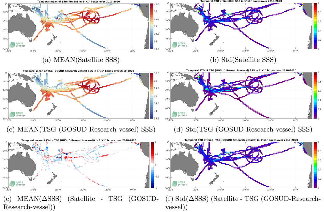
Figure 6: Temporal mean (left) and Std (right) of SSS from SMOS SSS L3 v335 - Monthly - 25 km (CATDS-CPDC) (top), TSG (GOSUD-Research-vessel) (middle), and of \Delta SSS (Satellite - TSG (GOSUD-Research-vessel)). Only match-up pairs are used to generate these maps.
