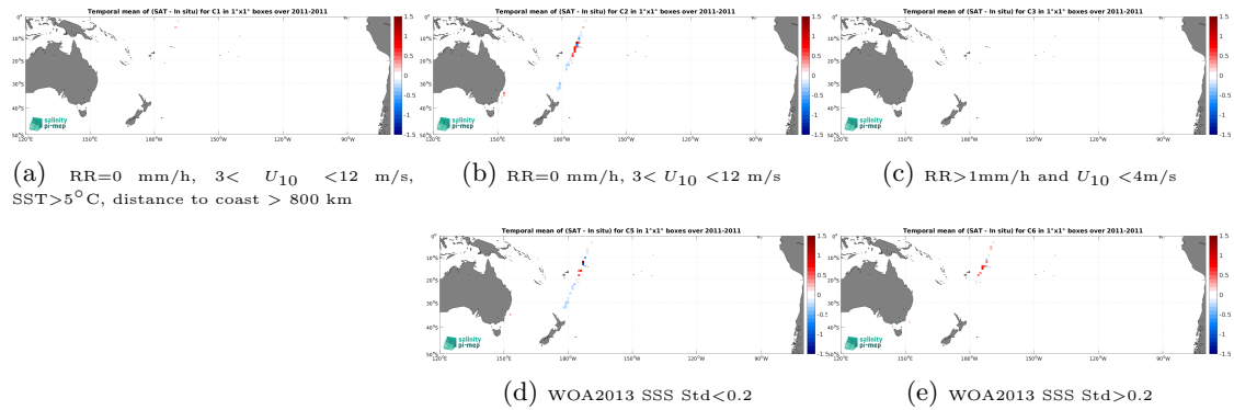
Figure 12: Temporal mean gridded over spatial boxes of size 1^{\circ}\times 1^{\circ} of \Delta\text{SSS} (SMOS SSS L3 v335 - Monthly - 25 km (CATDS-CPDC) - TSG (CSIC-UTM)) for 5 different subdatasets corresponding to: RR=0 mm/h, 3 < U_{10} < 12 m/s, SST > 5^{\circ}\text{C} , distance to coast > 800 km (a), RR=0 mm/h, 3 < U_{10} < 12 m/s (b), RR > 1 mm/h and U_{10} < 4 m/s (c), WOA2013 SSS Std < 0.2 (d), WOA2013 SSS Std > 0.2 (e).
