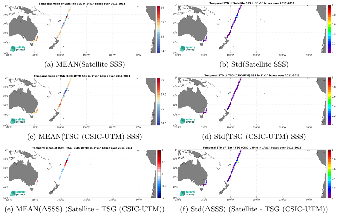
Figure 6: Temporal mean (left) and Std (right) of SSS from SMOS SSS L3 v335 - Monthly - 25 km (CATDS-CPDC) (top), TSG (CSIC-UTM) (middle), and of \Delta SSS (Satellite - TSG (CSIC-UTM)). Only match-up pairs are used to generate these maps.
