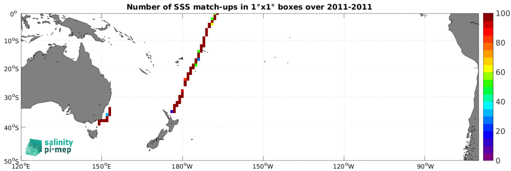
Figure 4: Number of SSS match-ups between TSG (CSIC-UTM) SSS and the SMOS SSS L3 v335 - Monthly - 25 km (CATDS-CPDC) SSS product for the South Pacific Ocean Pi-MEP region over 1^\circ \times 1^\circ boxes and for the full satellite product period.
