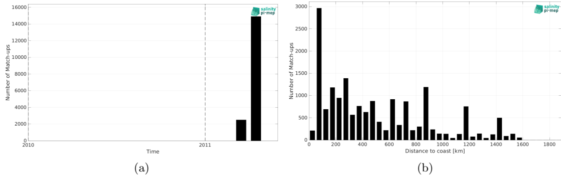
Figure 1: Number of match-ups between TSG (CSIC-UTM) and SMOS SSS L3 v335 - Monthly - 25 km (CATDS-CPDC) SSS as a function of time (a) and as function of the distance to coast (b) over the South Pacific Ocean Pi-MEP region and for the full satellite product period.
