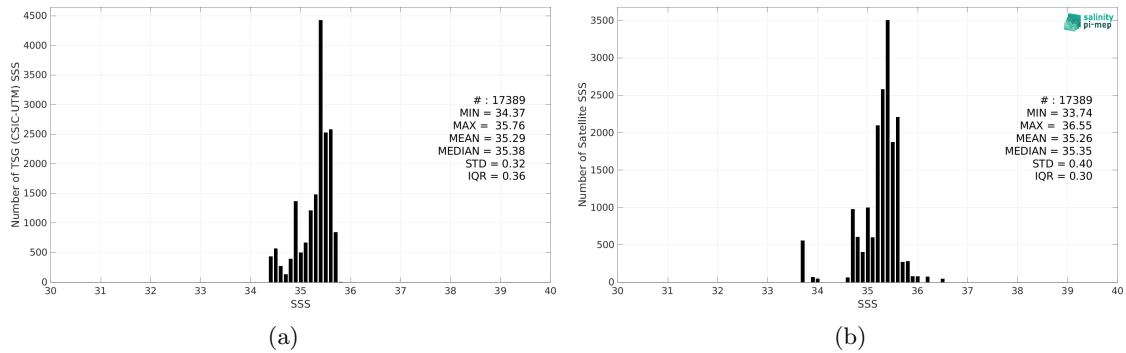
Figure 2: Histograms of SSS from TSG (CSIC-UTM) (a) and SMOS SSS L3 v335 - Monthly - 25 km (CATDS-CPDC) (b) considering all match-up pairs per bins of 0.1 over the South Pacific Ocean Pi-MEP region and for the full satellite product period.
