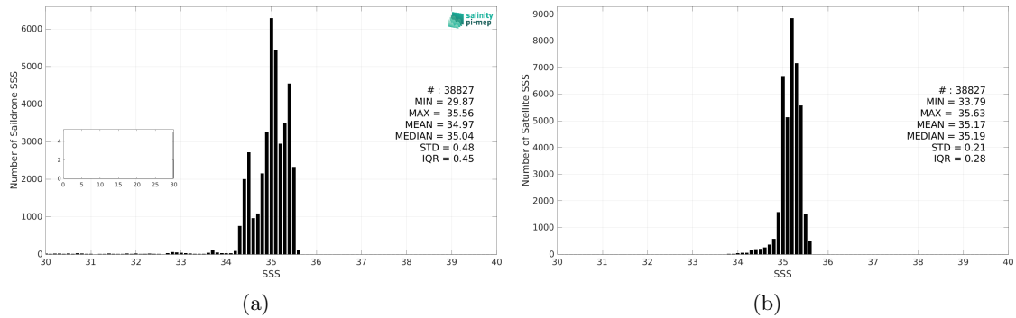
Figure 3: Histograms of SSS from Saildrone (a) and SMOS SSS L3 v335 - Monthly - 25 km (CATDS-CPDC) (b) considering all match-up pairs per bins of 0.1 over the South Pacific Ocean Pi-MEP region and for the full satellite product period.
