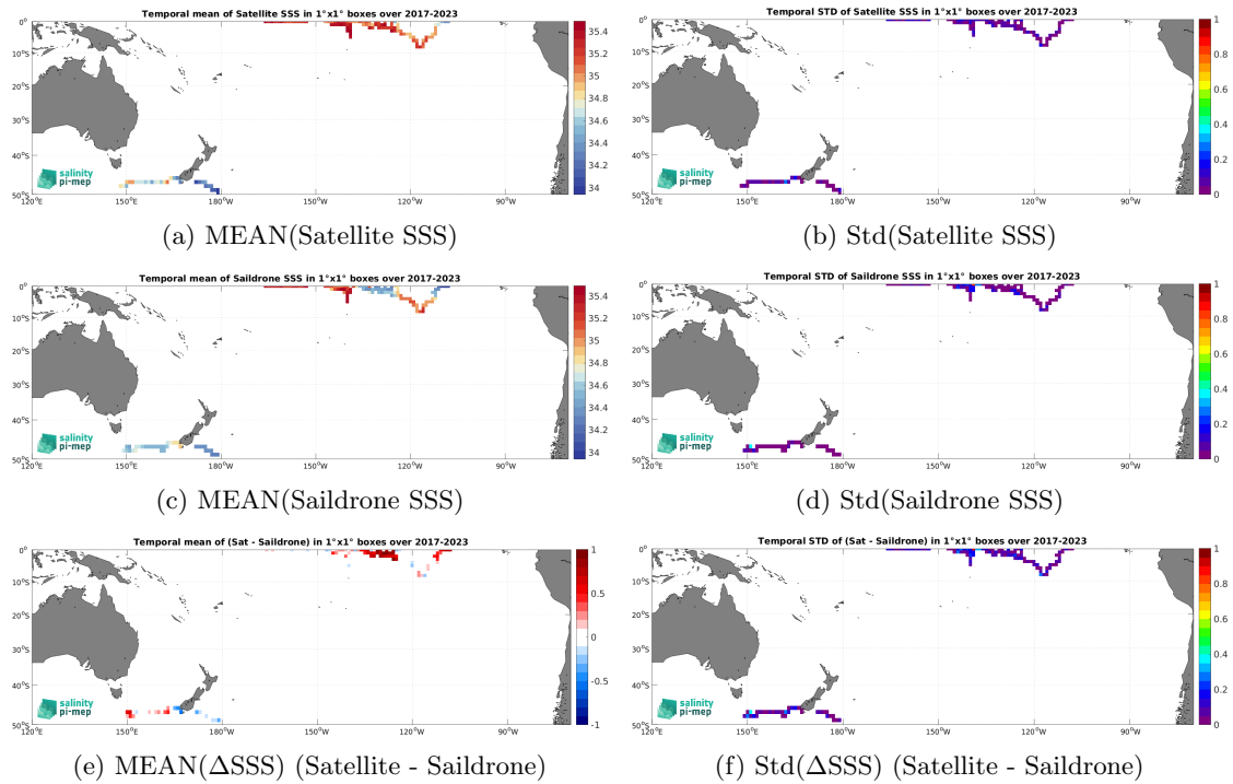
Figure 7: Temporal mean (left) and Std (right) of SSS from SMOS SSS L3 v335 - Monthly - 25 km (CATDS-CPDC) (top), Saildrone (middle), and of \Delta SSS (Satellite - Saildrone). Only match-up pairs are used to generate these maps.
