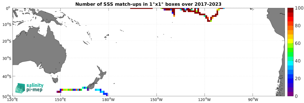
Figure 5: Number of SSS match-ups between Saildrone SSS and the SMOS SSS L3 v335 - Monthly - 25 km (CATDS-CPDC) SSS product for the South Pacific Ocean Pi-MEP region over 1^\circ \times 1^\circ boxes and for the full satellite product period.
