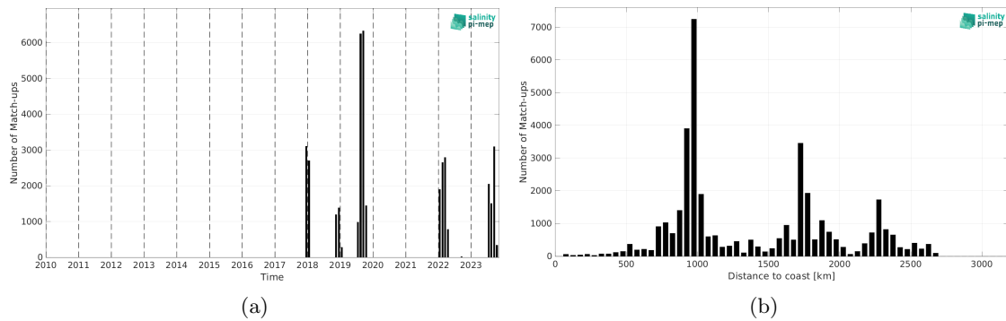
Figure 2: Number of match-ups between Saildrone and SMOS SSS L3 v335 - Monthly - 25 km (CATDS-CPDC) SSS as a function of time (a) and as function of the distance to coast (b) over the South Pacific Ocean Pi-MEP region and for the full satellite product period.
