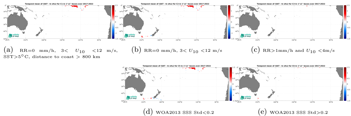
Figure 14: Temporal mean gridded over spatial boxes of size 1^\circ \times 1^\circ of \Delta\text{SSS} (SMOS SSS L3 v335 - Monthly - 25 km (CATDS-CPDC) - Saildrone) for 5 different subdatasets corresponding to:RR=0 mm/h, 3 < U_{10} < 12 m/s, SST>5°C, distance to coast > 800 km (a), RR=0 mm/h, 3 < U_{10} < 12 m/s (b), RR>1mm/h and U_{10} < 4 m/s (c), WOA2013 SSS Std<0.2 (d), WOA2013 SSS Std>0.2 (e).
