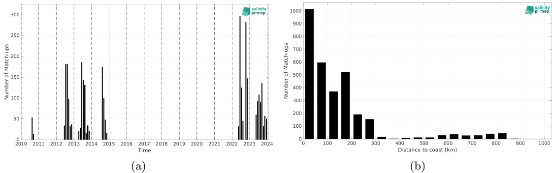
Figure 2: Number of match-ups between Marine mammals and SMOS SSS L3 v335 - Monthly - 25 km (CATDS-CPDC) SSS as a function of time (a) and as function of the distance to coast (b) over the South Pacific Ocean Pi-MEP region and for the full satellite product period.
