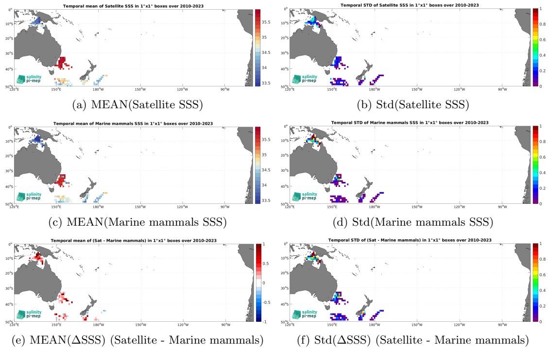
Figure 7: Temporal mean (left) and Std (right) of SSS from SMOS SSS L3 v335 - Monthly - 25 km (CATDS-CPDC) (top), Marine mammals (middle), and of \Delta SSS (Satellite - Marine mammals). Only match-up pairs are used to generate these maps.
