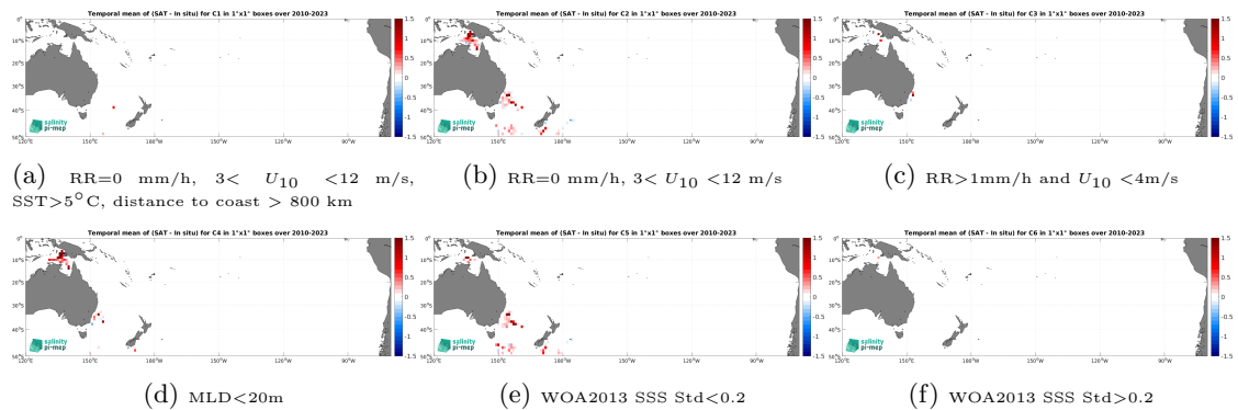
Figure 14: Temporal mean gridded over spatial boxes of size 1^\circ \times 1^\circ of \Delta SSS (SMOS SSS L3 v335 - Monthly - 25 km (CATDS-CPDC) - Marine mammals) for 6 different subdatasets corresponding to:RR=0 mm/h, 3 < U_{10} < 12 m/s, SST >5^\circ C, distance to coast > 800 km (a), RR=0 mm/h, 3 < U_{10} < 12 m/s (b), RR >1 mm/h and U_{10} < 4 m/s (c),MLD <20 m (d),WOA2013 SSS Std <0.2 (e),WOA2013 SSS Std >0.2 (f).
