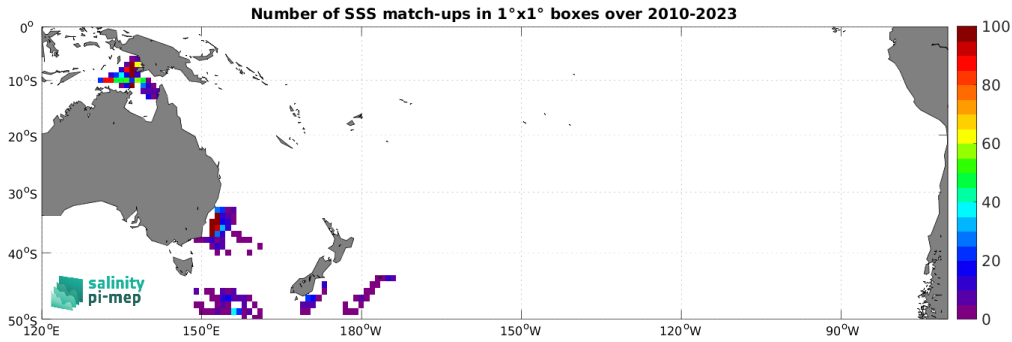
Figure 5: Number of SSS match-ups between Marine mammals SSS and the SMOS SSS L3 v335 - Monthly - 25 km (CATDS-CPDC) SSS product for the South Pacific Ocean Pi-MEP region over 1^\circ \times 1^\circ boxes and for the full satellite product period.
