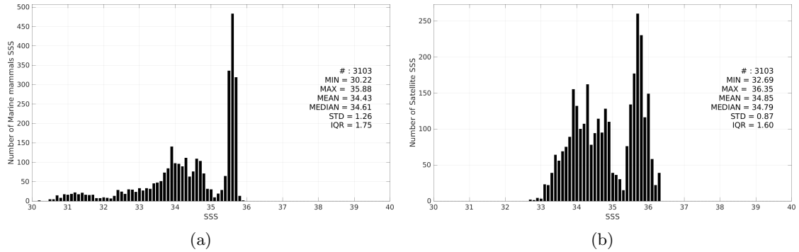
Figure 3: Histograms of SSS from Marine mammals (a) and SMOS SSS L3 v335 - Monthly - 25 km (CATDS-CPDC) (b) considering all match-up pairs per bins of 0.1 over the South Pacific Ocean Pi-MEP region and for the full satellite product period.
