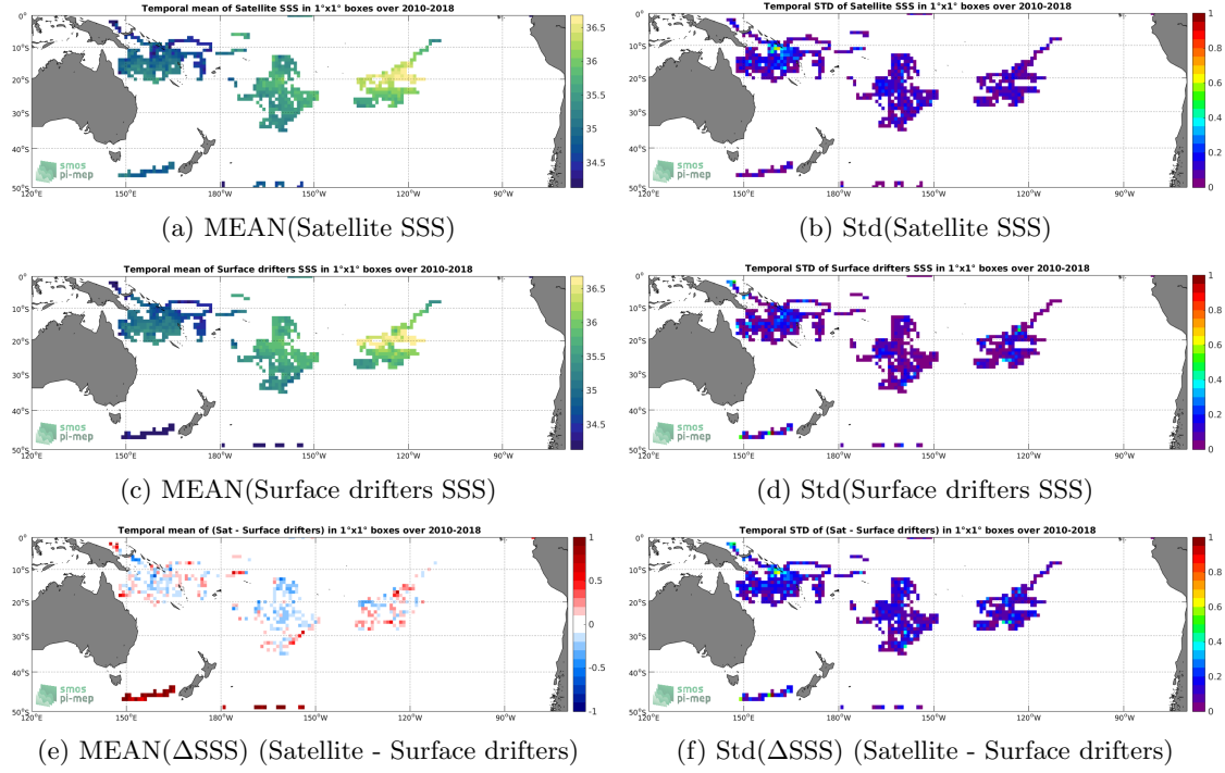
Figure 5: Temporal mean (left) and Std (right) of SSS from SMOS SSS L3 v335 - Monthly - 25 km (CATDS-CPDC) (top), Surface drifters (middle), and of \Delta\text{SSS} (Satellite - Surface drifters). Only match-up pairs are used to generate these maps.
