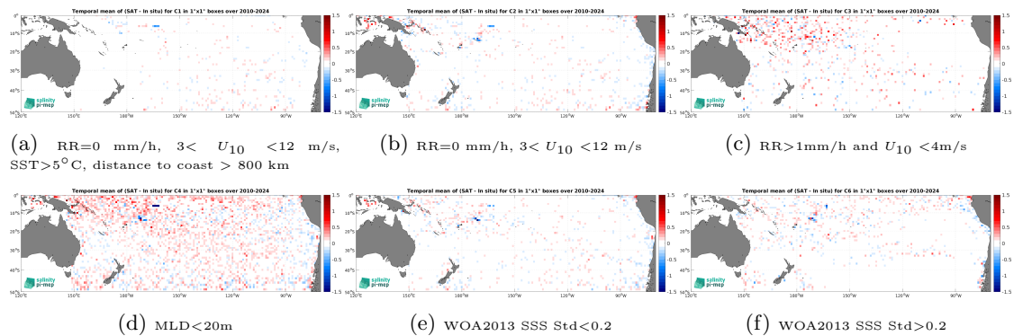
Figure 14: Temporal mean gridded over spatial boxes of size 1^\circ \times 1^\circ of \Delta SSS (SMOS SSS L3 v335 - Monthly - 25 km (CATDS-CPDC) - Argo) for 6 different subdatasets corresponding to:RR=0 mm/h, 3 < U_{10} < 12 m/s, SST >5^\circ\text{C} , distance to coast > 800 km (a), RR=0 mm/h, 3 < U_{10} < 12 m/s (b), RR >1 mm/h and U_{10} < 4 m/s (c),MLD <20 m (d),WOA2013 SSS Std <0.2 (e),WOA2013 SSS Std >0.2 (f).
