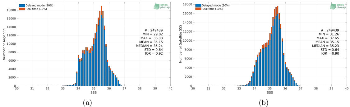
Figure 2: Histograms of SSS from Argo (a) and SMOS SSS L3 v335 - Monthly - 25 km (CATDS-CPDC) (b) considering all match-up pairs per bins of 0.1 over the South Pacific Ocean Pi-MEP region and for the full satellite product period.
