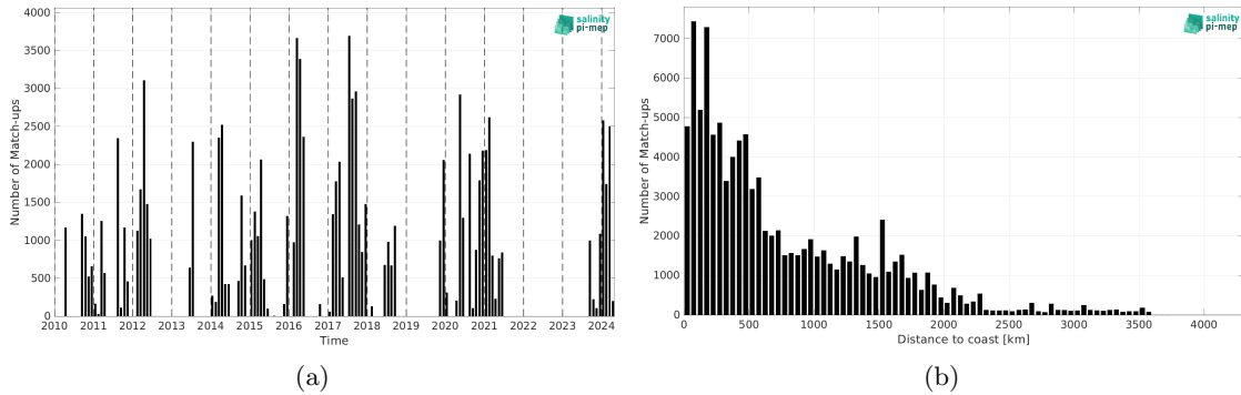
Figure 2: Number of match-ups between TSG (SAMOS) and SMOS SSS L3 v335 - 10 Days - 25 km (CATDS-CPDC) SSS as a function of time (a) and as function of the distance to coast (b) over the South Pacific Ocean Pi-MEP region and for the full satellite product period.
