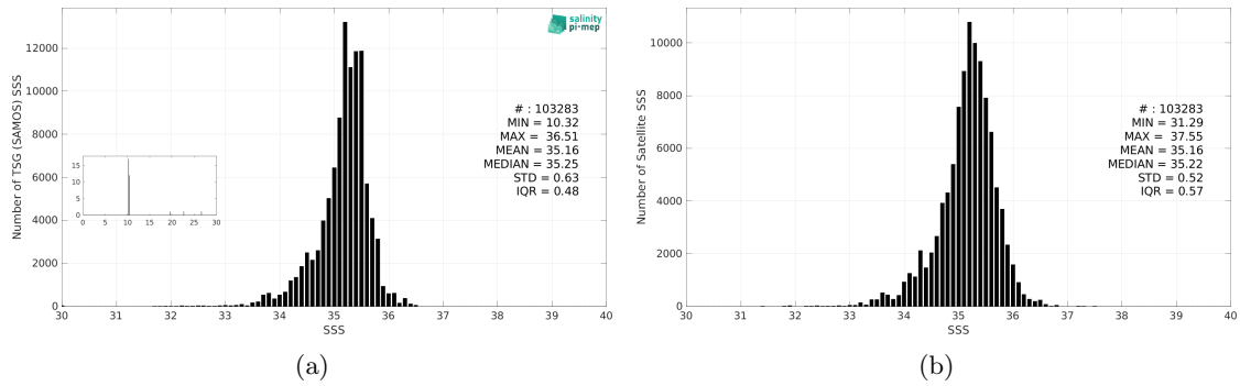
Figure 3: Histograms of SSS from TSG (SAMOS) (a) and SMOS SSS L3 v335 - 10 Days - 25 km (CATDS-CPDC) (b) considering all match-up pairs per bins of 0.1 over the South Pacific Ocean Pi-MEP region and for the full satellite product period.
