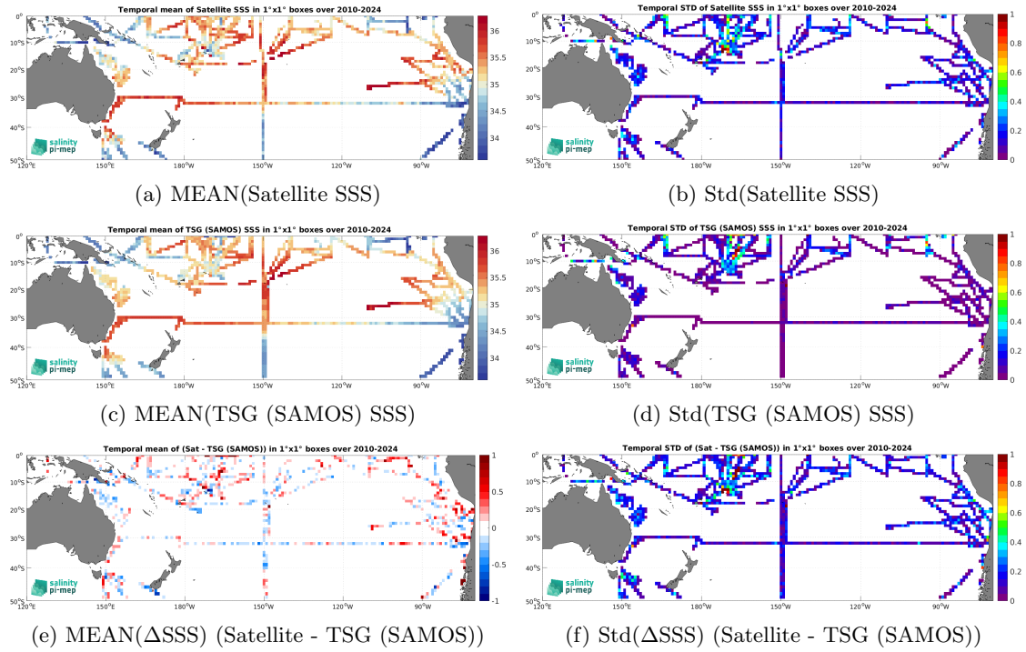
Figure 7: Temporal mean (left) and Std (right) of SSS from SMOS SSS L3 v335 - 10 Days - 25 km (CATDS-CPDC) (top), TSG (SAMOS) (middle), and of \Delta SSS (Satellite - TSG (SAMOS)). Only match-up pairs are used to generate these maps.
