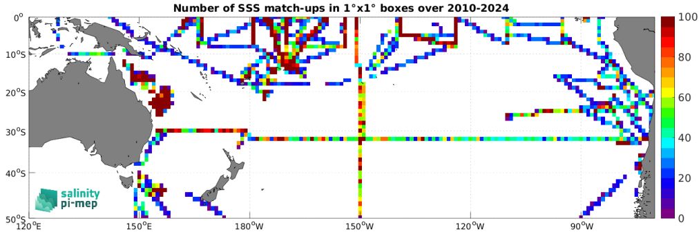
Figure 5: Number of SSS match-ups between TSG (SAMOS) SSS and the SMOS SSS L3 v335 - 10 Days - 25 km (CATDS-CPDC) SSS product for the South Pacific Ocean Pi-MEP region over 1^\circ \times 1^\circ boxes and for the full satellite product period.
