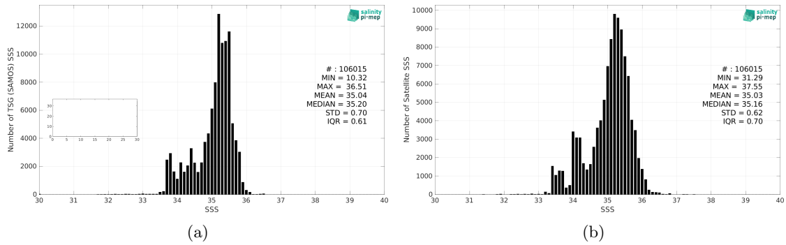
Figure 2: Histograms of SSS from TSG (SAMOS) (a) and SMOS SSS L3 v335 - 10 Days - 25 km (CATDS-CPDC) (b) considering all match-up pairs per bins of 0.1 over the South Pacific Ocean Pi-MEP region and for the full satellite product period.
