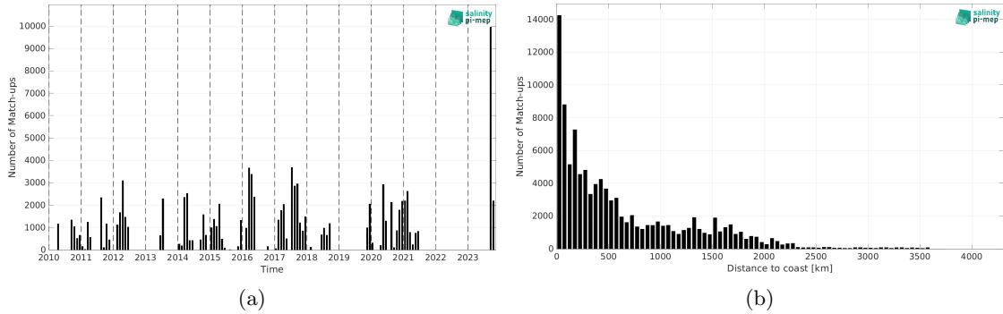
Figure 1: Number of match-ups between TSG (SAMOS) and SMOS SSS L3 v335 - 10 Days - 25 km (CATDS-CPDC) SSS as a function of time (a) and as function of the distance to coast (b) over the South Pacific Ocean Pi-MEP region and for the full satellite product period.
