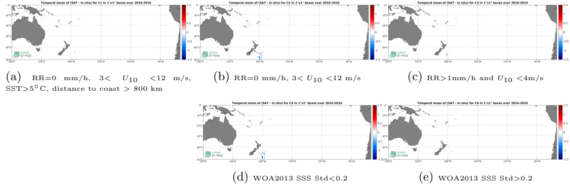
Figure 12: Temporal mean gridded over spatial boxes of size 1^{\circ} \times 1^{\circ} of \Delta\text{SSS} (SMOS SSS L3 v335 - 10 Days - 25 km (CATDS-CPDC) - TSG (Polarstern)) for 5 different subdatasets corresponding to: \text{RR}=0 mm/h, 3 < U_{10} < 12 m/s, SST > 5^{\circ}\text{C} , distance to coast > 800 km (a), \text{RR}=0 mm/h, 3 < U_{10} < 12 m/s (b), \text{RR} > 1 mm/h and U_{10} < 4 m/s (c), WOA2013 SSS Std < 0.2 (d), WOA2013 SSS Std > 0.2 (e).
