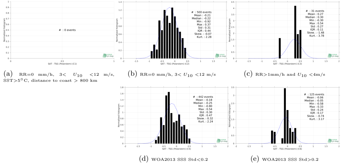
Figure 13: Normalized histogram of \Delta\text{SSS} (SMOS SSS L3 v335 - 10 Days - 25 km (CATDS-CPDC) - TSG (Polarstern)) for 5 different subdatasets corresponding to: RR=0 mm/h, 3 < U_{10} < 12 m/s, SST > 5^\circ\text{C} , distance to coast > 800 km (a), RR=0 mm/h, 3 < U_{10} < 12 m/s (b), RR > 1 mm/h and U_{10} < 4 m/s (c), WOA2013 SSS Std < 0.2 (d), WOA2013 SSS Std > 0.2 (e).
