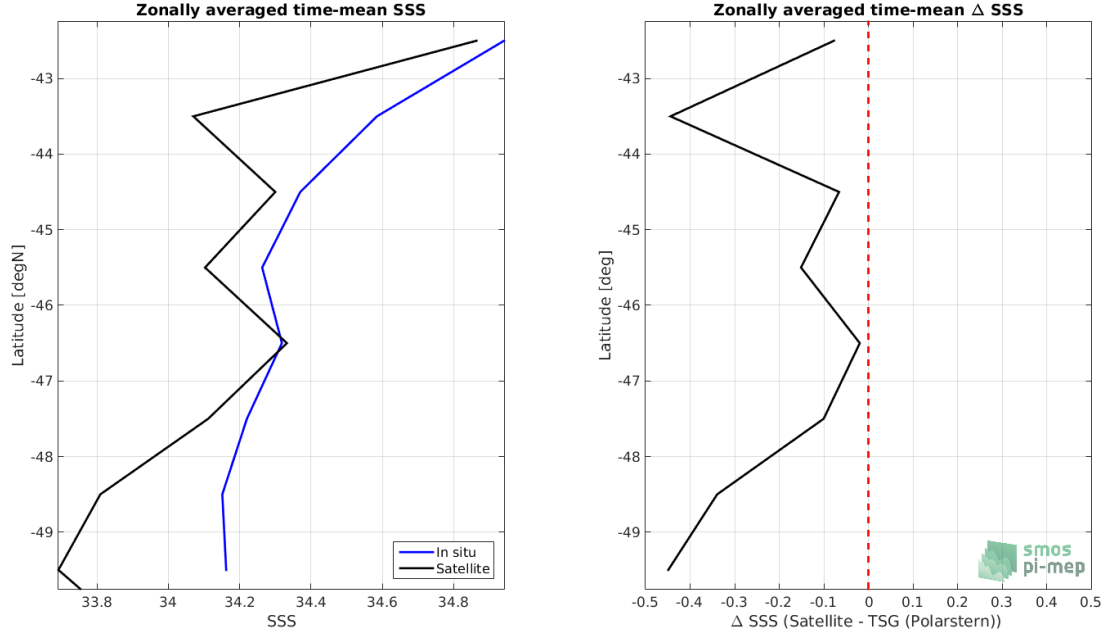
Figure 8: Left panel: Zonal mean SSS from SMOS SSS L3 v335 - 10 Days - 25 km (CATDS-CPDC) satellite product (black) and from TSG (Polarstern) (blue). Right panel: Zonal mean of \Delta\text{SSS} (Satellite - TSG (Polarstern)) for all the collected Pi-MEP match-up pairs estimated over the full satellite product period.
