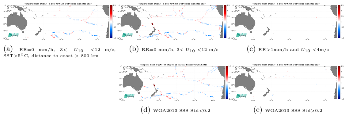
Figure 14: Temporal mean gridded over spatial boxes of size 1^\circ \times 1^\circ of \Delta\text{SSS} (SMOS SSS L3 v335 - 10 Days - 25 km (CATDS-CPDC) - TSG (GOSUD-Sailing-ship)) for 5 different subdatasets corresponding to:RR=0 mm/h, 3 < U_{10} < 12 m/s, SST>5°C, distance to coast > 800 km (a), RR=0 mm/h, 3 < U_{10} < 12 m/s (b), RR>1mm/h and U_{10} < 4 m/s (c), WOA2013 SSS Std<0.2 (d), WOA2013 SSS Std>0.2 (e).
