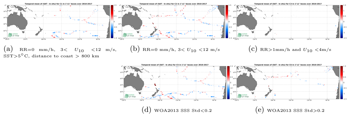
Figure 12: Temporal mean gridded over spatial boxes of size 1^\circ \times 1^\circ of \Delta\text{SSS} (SMOS SSS L3 v335 - 10 Days - 25 km (CATDS-CPDC) - TSG (GOSUD-Sailing-ship)) for 5 different subdatasets corresponding to:RR=0 mm/h, 3 < U_{10} < 12 m/s, SST>5°C, distance to coast > 800 km (a), RR=0 mm/h, 3 < U_{10} < 12 m/s (b), RR>1mm/h and U_{10} < 4 m/s (c), WOA2013 SSS Std<0.2 (d), WOA2013 SSS Std>0.2 (e).
