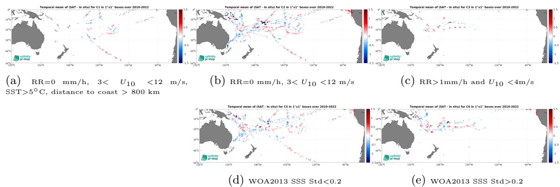
Figure 14: Temporal mean gridded over spatial boxes of size 1^\circ \times 1^\circ of \Delta SSS (SMOS SSS L3 v335 - 10 Days - 25 km (CATDS-CPDC) - TSG (GOSUD-Research-vessel)) for 5 different subdatasets corresponding to:RR=0 mm/h, 3 < U_{10} < 12 m/s, SST >5^\circ C, distance to coast > 800 km (a), RR=0 mm/h, 3 < U_{10} < 12 m/s (b), RR >1 mm/h and U_{10} < 4 m/s (c), WOA2013 SSS Std <0.2 (d), WOA2013 SSS Std >0.2 (e).
