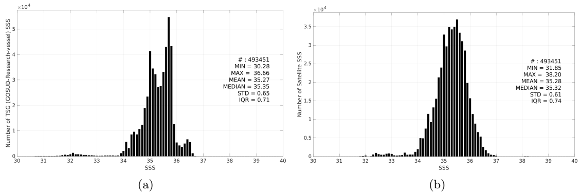
Figure 3: Histograms of SSS from TSG (GOSUD-Research-vessel) (a) and SMOS SSS L3 v335 - 10 Days - 25 km (CATDS-CPDC) (b) considering all match-up pairs per bins of 0.1 over the South Pacific Ocean Pi-MEP region and for the full satellite product period.
