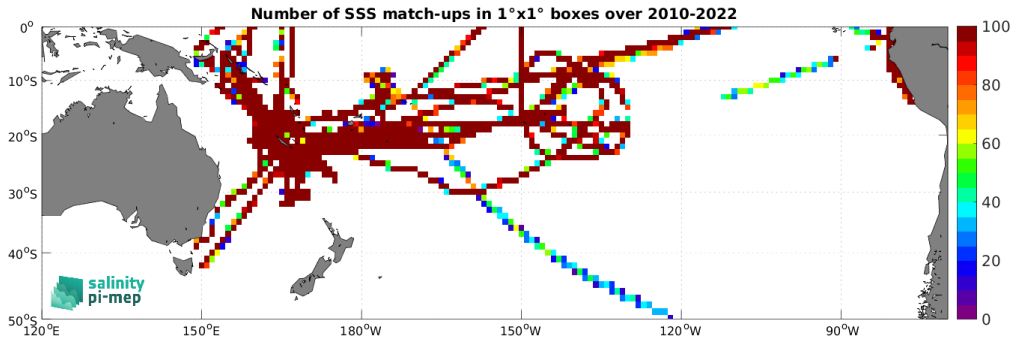
Figure 5: Number of SSS match-ups between TSG (GOSUD-Research-vessel) SSS and the SMOS SSS L3 v335 - 10 Days - 25 km (CATDS-CPDC) SSS product for the South Pacific Ocean Pi-MEP region over 1^\circ \times 1^\circ boxes and for the full satellite product period.
