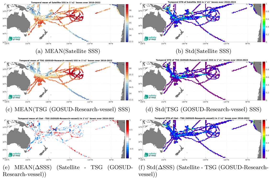
Figure 7: Temporal mean (left) and Std (right) of SSS from SMOS SSS L3 v335 - 10 Days - 25 km (CATDS-CPDC) (top), TSG (GOSUD-Research-vessel) (middle), and of \Delta SSS (Satellite - TSG (GOSUD-Research-vessel)). Only match-up pairs are used to generate these maps.
