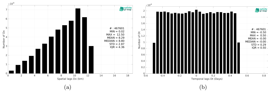
Figure 6: Histograms of the spatial (a) and temporal (b) lags between the location/time of the TSG (GOSUD-Research-vessel) measurement and the date of the corresponding SMOS SSS L3 v335 - 10 Days - 25 km (CATDS-CPDC) SSS pixel.
