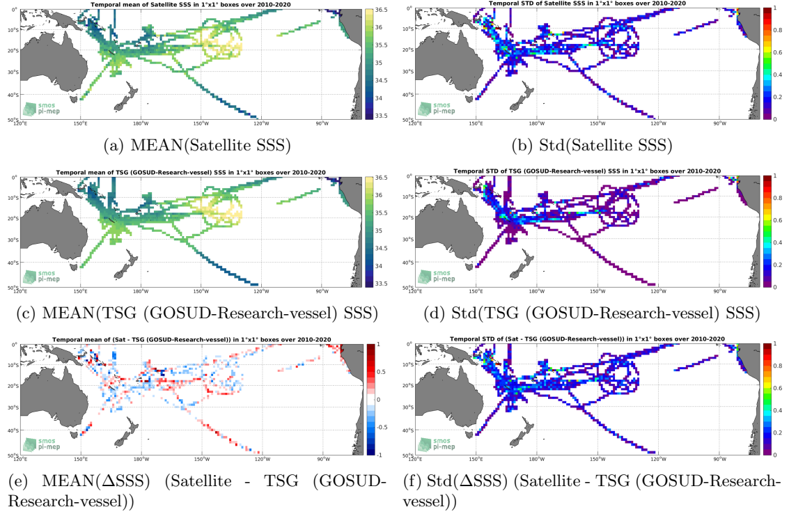
Figure 6: Temporal mean (left) and Std (right) of SSS from SMOS SSS L3 v335 - 10 Days - 25 km (CATDS-CPDC) (top), TSG (GOSUD-Research-vessel) (middle), and of \Delta SSS (Satellite - TSG (GOSUD-Research-vessel)). Only match-up pairs are used to generate these maps.
