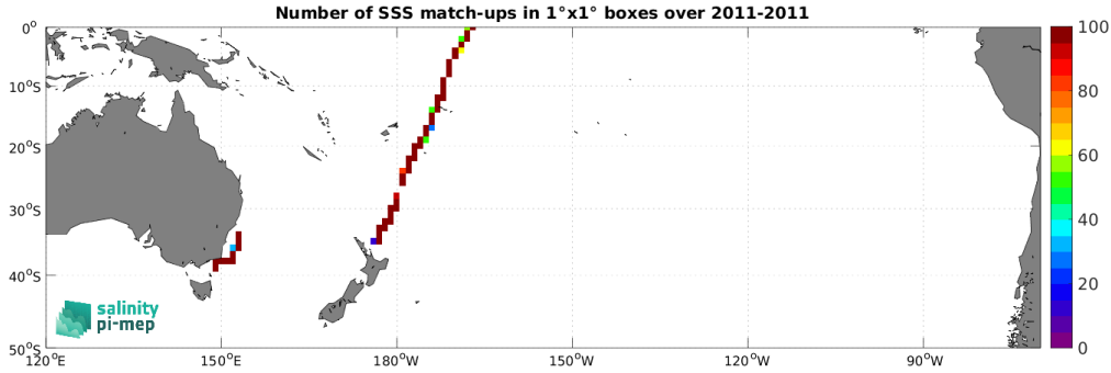
Figure 5: Number of SSS match-ups between TSG (CSIC-UTM) SSS and the SMOS SSS L3 v335 - 10 Days - 25 km (CATDS-CPDC) SSS product for the South Pacific Ocean Pi-MEP region over 1^\circ \times 1^\circ boxes and for the full satellite product period.
