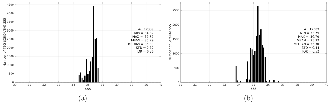
Figure 3: Histograms of SSS from TSG (CSIC-UTM) (a) and SMOS SSS L3 v335 - 10 Days - 25 km (CATDS-CPDC) (b) considering all match-up pairs per bins of 0.1 over the South Pacific Ocean Pi-MEP region and for the full satellite product period.
