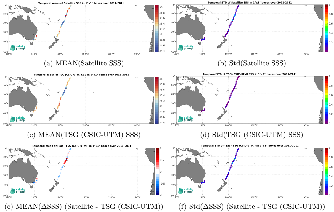
Figure 7: Temporal mean (left) and Std (right) of SSS from SMOS SSS L3 v335 - 10 Days - 25 km (CATDS-CPDC) (top), TSG (CSIC-UTM) (middle), and of \Delta SSS (Satellite - TSG (CSIC-UTM)). Only match-up pairs are used to generate these maps.
