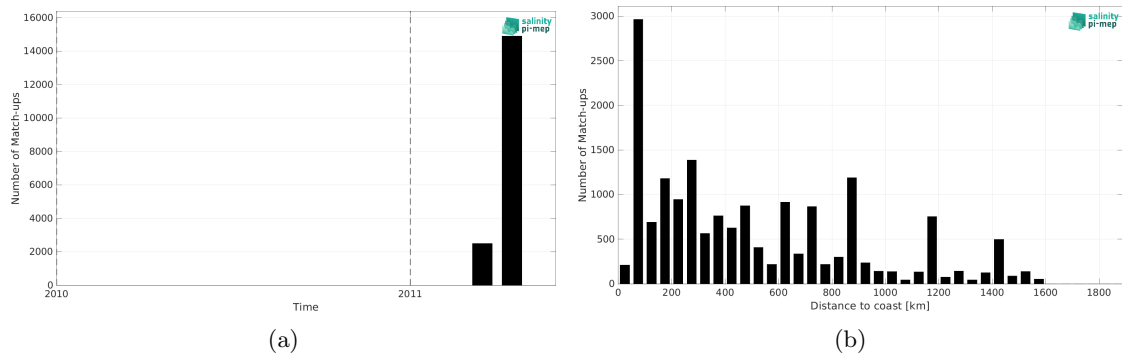
Figure 2: Number of match-ups between TSG (CSIC-UTM) and SMOS SSS L3 v335 - 10 Days - 25 km (CATDS-CPDC) SSS as a function of time (a) and as function of the distance to coast (b) over the South Pacific Ocean Pi-MEP region and for the full satellite product period.
