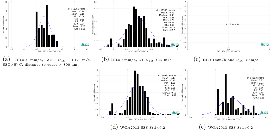
Figure 13: Normalized histogram of \Delta\text{SSS} (SMOS SSS L3 v335 - 10 Days - 25 km (CATDS-CPDC) - TSG (CSIC-UTM)) for 5 different subdatasets corresponding to: RR=0 mm/h, 3 < U_{10} < 12 m/s, SST>5°C, distance to coast > 800 km (a), RR=0 mm/h, 3 < U_{10} < 12 m/s (b), RR>1mm/h and U_{10} < 4 m/s (c), WOA2013 SSS Std<0.2 (d), WOA2013 SSS Std>0.2 (e).
