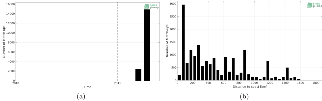
Figure 1: Number of match-ups between TSG (CSIC-UTM) and SMOS SSS L3 v335 - 10 Days - 25 km (CATDS-CPDC) SSS as a function of time (a) and as function of the distance to coast (b) over the South Pacific Ocean Pi-MEP region and for the full satellite product period.
