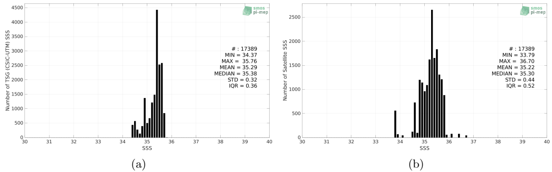
Figure 2: Histograms of SSS from TSG (CSIC-UTM) (a) and SMOS SSS L3 v335 - 10 Days - 25 km (CATDS-CPDC) (b) considering all match-up pairs per bins of 0.1 over the South Pacific Ocean Pi-MEP region and for the full satellite product period.
