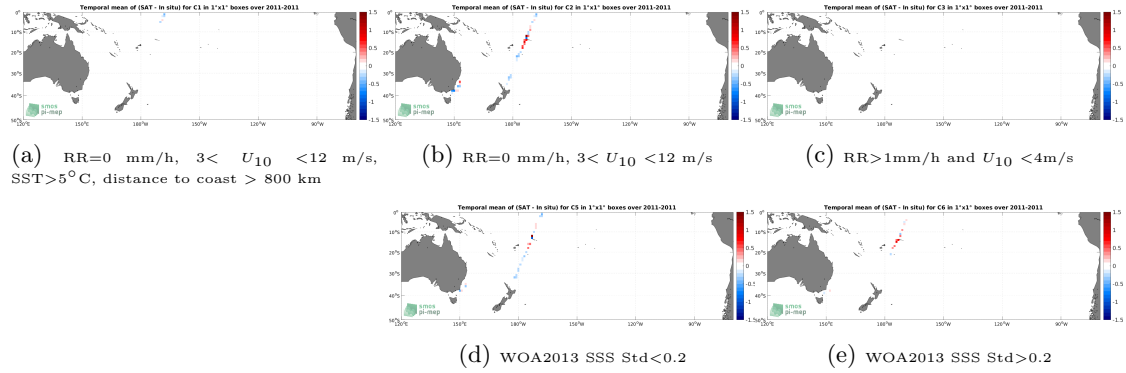
Figure 12: Temporal mean gridded over spatial boxes of size 1^{\circ}\times 1^{\circ} of \Delta\text{SSS} (SMOS SSS L3 v335 - 10 Days - 25 km (CATDS-CPDC) - TSG (CSIC-UTM)) for 5 different subdatasets corresponding to:RR=0 mm/h, 3 < U_{10} < 12 m/s, SST > 5^{\circ}\text{C} , distance to coast > 800 km (a), RR=0 mm/h, 3 < U_{10} < 12 m/s (b), RR > 1 mm/h and U_{10} < 4 m/s (c), WOA2013 SSS Std < 0.2 (d), WOA2013 SSS Std > 0.2 (e).
