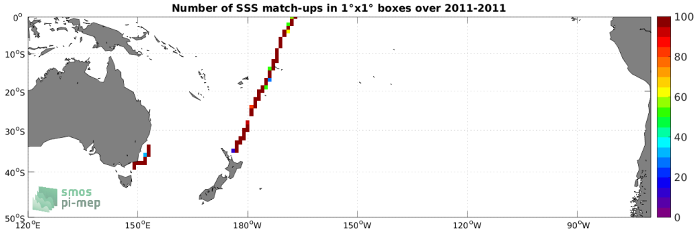
Figure 4: Number of SSS match-ups between TSG (CSIC-UTM) SSS and the SMOS SSS L3 v335 - 10 Days - 25 km (CATDS-CPDC) SSS product for the South Pacific Ocean Pi-MEP region over 1^\circ \times 1^\circ boxes and for the full satellite product period.
