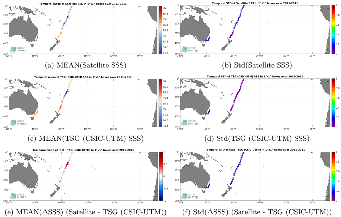
Figure 6: Temporal mean (left) and Std (right) of SSS from SMOS SSS L3 v335 - 10 Days - 25 km (CATDS-CPDC) (top), TSG (CSIC-UTM) (middle), and of \Delta SSS (Satellite - TSG (CSIC-UTM)). Only match-up pairs are used to generate these maps.
