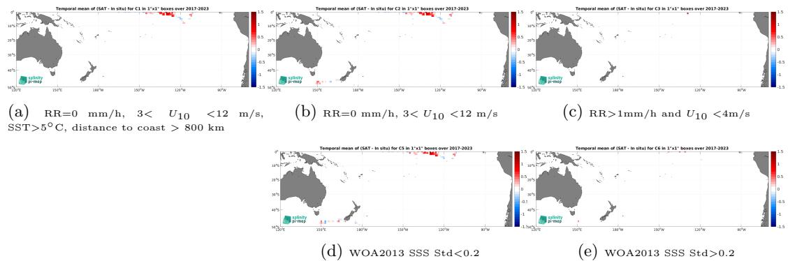
Figure 14: Temporal mean gridded over spatial boxes of size 1^\circ \times 1^\circ of \Delta\text{SSS} (SMOS SSS L3 v335 - 10 Days - 25 km (CATDS-CPDC) - Saildrone) for 5 different subdatasets corresponding to:RR=0 mm/h, 3 < U_{10} < 12 m/s, SST>5°C, distance to coast > 800 km (a), RR=0 mm/h, 3 < U_{10} < 12 m/s (b), RR>1mm/h and U_{10} < 4 m/s (c), WOA2013 SSS Std<0.2 (d), WOA2013 SSS Std>0.2 (e).
