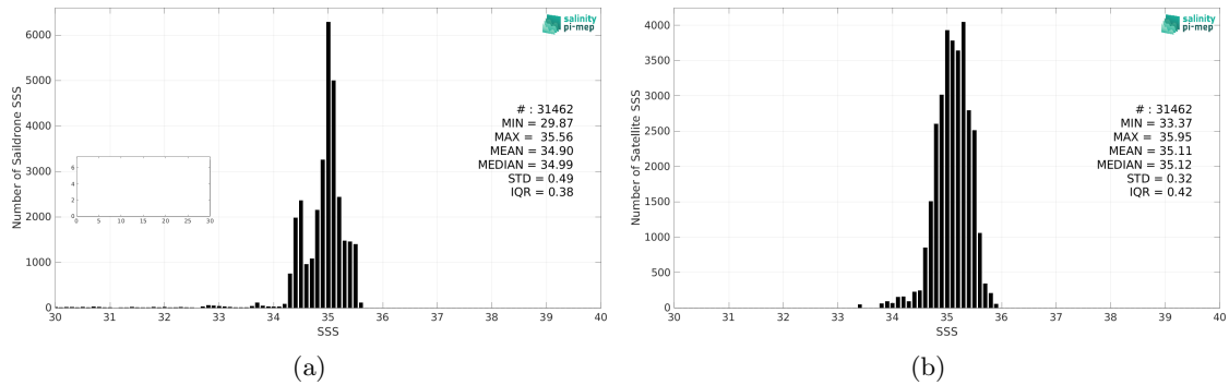
Figure 2: Histograms of SSS from Saildrone (a) and SMOS SSS L3 v335 - 10 Days - 25 km (CATDS-CPDC) (b) considering all match-up pairs per bins of 0.1 over the South Pacific Ocean Pi-MEP region and for the full satellite product period.
