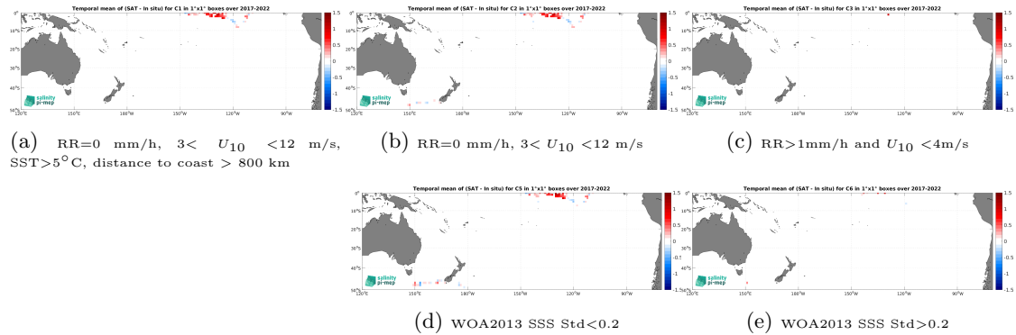
Figure 12: Temporal mean gridded over spatial boxes of size 1^\circ \times 1^\circ of \Delta SSS (SMOS SSS L3 v335 - 10 Days - 25 km (CATDS-CPDC) - Saildrone) for 5 different subdatasets corresponding to:RR=0 mm/h, 3 < U_{10} < 12 m/s, SST >5^\circ C, distance to coast > 800 km (a), RR=0 mm/h, 3 < U_{10} < 12 m/s (b), RR >1 mm/h and U_{10} < 4 m/s (c), WOA2013 SSS Std <0.2 (d), WOA2013 SSS Std >0.2 (e).
