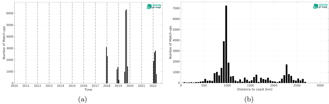
Figure 1: Number of match-ups between Saildrone and SMOS SSS L3 v335 - 10 Days - 25 km (CATDS-CPDC) SSS as a function of time (a) and as function of the distance to coast (b) over the South Pacific Ocean Pi-MEP region and for the full satellite product period.
