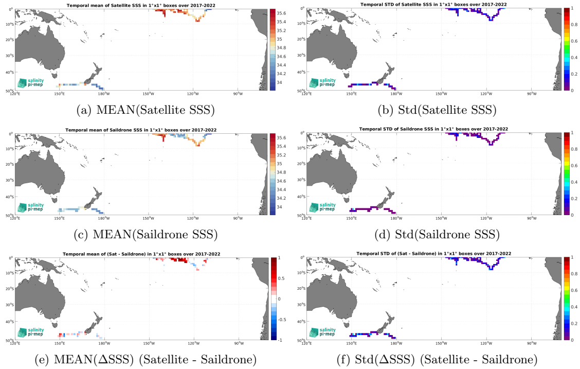
Figure 6: Temporal mean (left) and Std (right) of SSS from SMOS SSS L3 v335 - 10 Days - 25 km (CATDS-CPDC) (top), Saildrone (middle), and of \Delta SSS (Satellite - Saildrone). Only match-up pairs are used to generate these maps.
