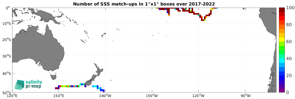
Figure 4: Number of SSS match-ups between Saildrone SSS and the SMOS SSS L3 v335 - 10 Days - 25 km (CATDS-CPDC) SSS product for the South Pacific Ocean Pi-MEP region over 1^\circ \times 1^\circ boxes and for the full satellite product period.
