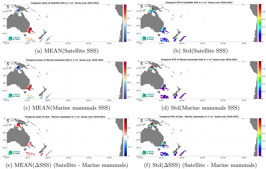
Figure 7: Temporal mean (left) and Std (right) of SSS from SMOS SSS L3 v335 - 10 Days - 25 km (CATDS-CPDC) (top), Marine mammals (middle), and of \Delta SSS (Satellite - Marine mammals). Only match-up pairs are used to generate these maps.
