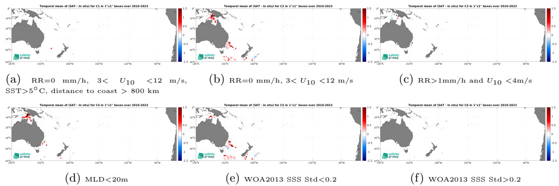
Figure 14: Temporal mean gridded over spatial boxes of size 1^\circ \times 1^\circ of \Delta SSS (SMOS SSS L3 v335 - 10 Days - 25 km (CATDS-CPDC) - Marine mammals) for 6 different subdatasets corresponding to:RR=0 mm/h, 3 < U_{10} < 12 m/s, SST >5^\circ C, distance to coast > 800 km (a), RR=0 mm/h, 3 < U_{10} < 12 m/s (b), RR >1 mm/h and U_{10} < 4 m/s (c),MLD <20 m (d),WOA2013 SSS Std <0.2 (e),WOA2013 SSS Std >0.2 (f).
