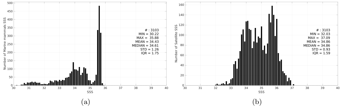
Figure 3: Histograms of SSS from Marine mammals (a) and SMOS SSS L3 v335 - 10 Days - 25 km (CATDS-CPDC) (b) considering all match-up pairs per bins of 0.1 over the South Pacific Ocean Pi-MEP region and for the full satellite product period.
