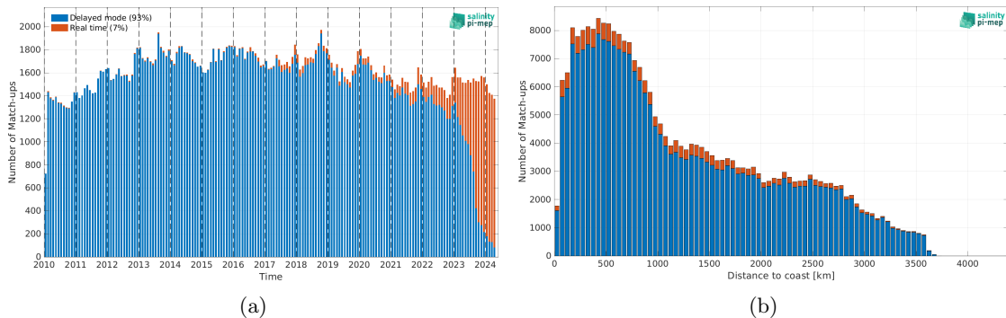
Figure 2: Number of match-ups between Argo and SMOS SSS L3 v335 - 10 Days - 25 km (CATDS-CPDC) SSS as a function of time (a) and as function of the distance to coast (b) over the South Pacific Ocean Pi-MEP region and for the full satellite product period.
