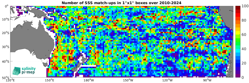
Figure 5: Number of SSS match-ups between Argo SSS and the SMOS SSS L3 v335 - 10 Days - 25 km (CATDS-CPDC) SSS product for the South Pacific Ocean Pi-MEP region over 1^\circ \times 1^\circ boxes and for the full satellite product period.
