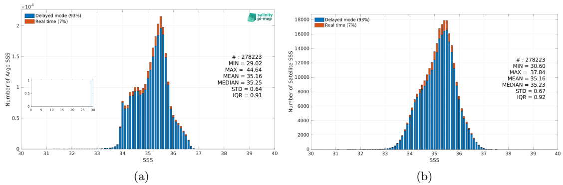
Figure 3: Histograms of SSS from Argo (a) and SMOS SSS L3 v335 - 10 Days - 25 km (CATDS-CPDC) (b) considering all match-up pairs per bins of 0.1 over the South Pacific Ocean Pi-MEP region and for the full satellite product period.
