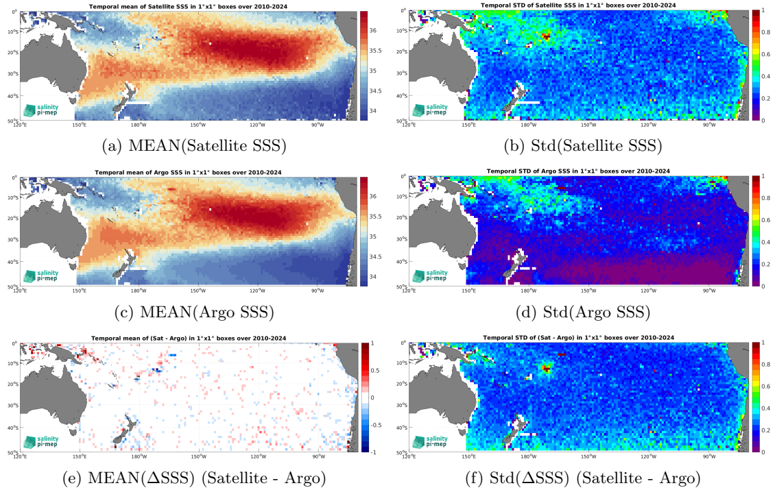
Figure 7: Temporal mean (left) and Std (right) of SSS from SMOS SSS L3 v335 - 10 Days - 25 km (CATDS-CPDC) (top), Argo (middle), and of \Delta SSS (Satellite - Argo). Only match-up pairs are used to generate these maps.
