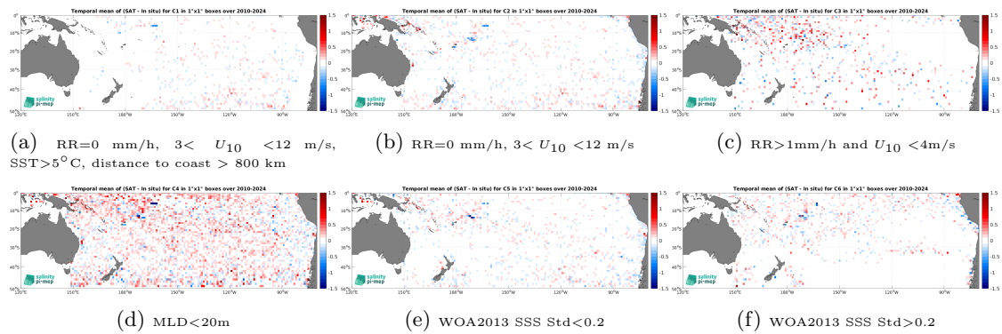
Figure 14: Temporal mean gridded over spatial boxes of size 1^\circ \times 1^\circ of \Delta SSS (SMOS SSS L3 v335 - 10 Days - 25 km (CATDS-CPDC) - Argo) for 6 different subdatasets corresponding to:RR=0 mm/h, 3 < U_{10} < 12 m/s, SST >5^\circ C, distance to coast > 800 km (a), RR=0 mm/h, 3 < U_{10} < 12 m/s (b), RR >1 mm/h and U_{10} < 4 m/s (c),MLD <20 m (d),WOA2013 SSS Std <0.2 (e),WOA2013 SSS Std >0.2 (f).
