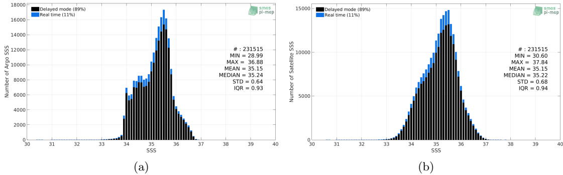
Figure 2: Histograms of SSS from Argo (a) and SMOS SSS L3 v335 - 10 Days - 25 km (CATDS-CPDC) (b) considering all match-up pairs per bins of 0.1 over the South Pacific Ocean Pi-MEP region and for the full satellite product period.
