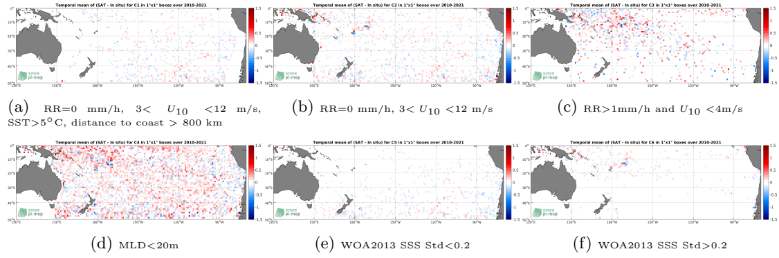
Figure 12: Temporal mean gridded over spatial boxes of size 1^\circ \times 1^\circ of \Delta SSS (SMOS SSS L3 v335 - 10 Days - 25 km (CATDS-CPDC) - Argo) for 6 different subdatasets corresponding to: RR=0 mm/h, 3 < U_{10} < 12 m/s, SST > 5^\circ C , distance to coast > 800 km (a), RR=0 mm/h, 3 < U_{10} < 12 m/s (b), RR > 1 mm/h and U_{10} < 4 m/s (c), MLD < 20 m (d), WOA2013 SSS Std < 0.2 (e), WOA2013 SSS Std > 0.2 (f).
