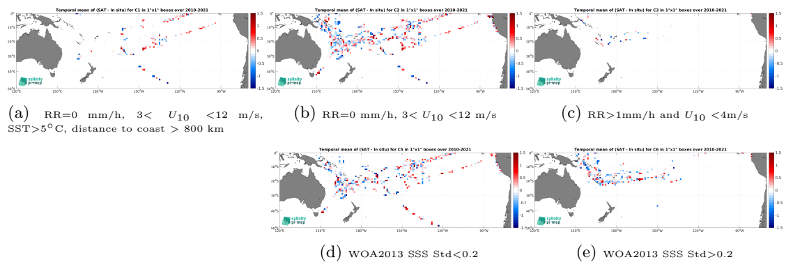
Figure 14: Temporal mean gridded over spatial boxes of size 1^\circ \times 1^\circ of \Delta\text{SSS} (SMOS SSS L2Q v333 - 0.25 Deg (CATDS-CPDC) - TSG (GOSUD-Research-vessel)) for 5 different subdatasets corresponding to:RR=0 mm/h, 3 < U_{10} < 12 m/s, SST>5°C, distance to coast > 800 km (a), RR=0 mm/h, 3 < U_{10} < 12 m/s (b), RR>1mm/h and U_{10} < 4 m/s (c), WOA2013 SSS Std<0.2 (d), WOA2013 SSS Std>0.2 (e).
