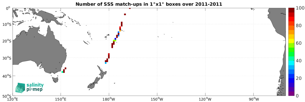
Figure 5: Number of SSS match-ups between TSG (CSIC-UTM) SSS and the SMOS SSS L2Q v333 - 0.25 Deg (CATDS-CPDC) SSS product for the South Pacific Ocean Pi-MEP region over 1^\circ \times 1^\circ boxes and for the full satellite product period.
