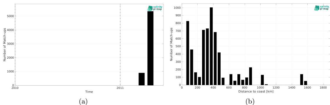
Figure 2: Number of match-ups between TSG (CSIC-UTM) and SMOS SSS L2Q v333 - 0.25 Deg (CATDS-CPDC) SSS as a function of time (a) and as function of the distance to coast (b) over the South Pacific Ocean Pi-MEP region and for the full satellite product period.
