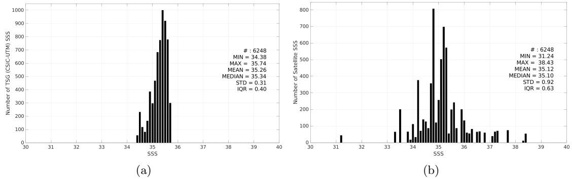
Figure 3: Histograms of SSS from TSG (CSIC-UTM) (a) and SMOS SSS L2Q v333 - 0.25 Deg (CATDS-CPDC) (b) considering all match-up pairs per bins of 0.1 over the South Pacific Ocean Pi-MEP region and for the full satellite product period.
