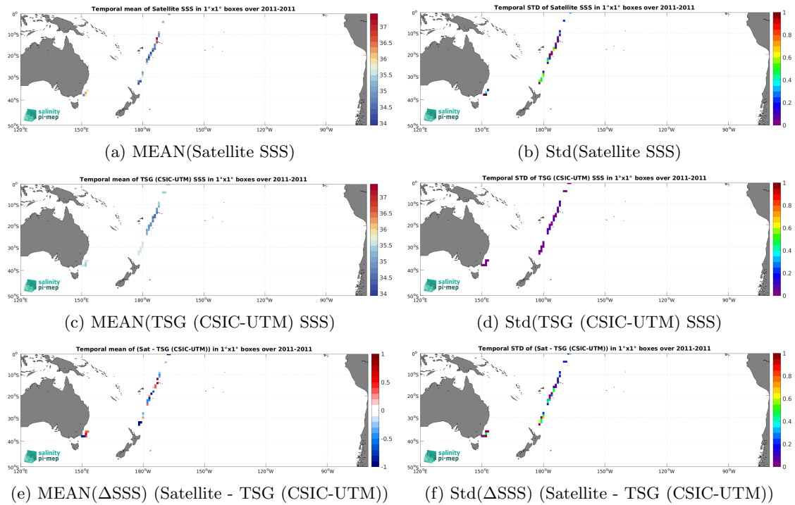
Figure 7: Temporal mean (left) and Std (right) of SSS from SMOS SSS L2Q v333 - 0.25 Deg (CATDS-CPDC) (top), TSG (CSIC-UTM) (middle), and of \Delta SSS (Satellite - TSG (CSIC-UTM)). Only match-up pairs are used to generate these maps.
