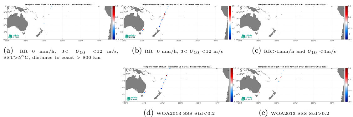
Figure 14: Temporal mean gridded over spatial boxes of size 1^\circ \times 1^\circ of \Delta SSS (SMOS SSS L2Q v333 - 0.25 Deg (CATDS-CPDC) - TSG (CSIC-UTM)) for 5 different subdatasets corresponding to:RR=0 mm/h, 3 < U_{10} < 12 m/s, SST>5°C, distance to coast > 800 km (a), RR=0 mm/h, 3 < U_{10} < 12 m/s (b), RR>1mm/h and U_{10} < 4 m/s (c), WOA2013 SSS Std<0.2 (d), WOA2013 SSS Std>0.2 (e).
